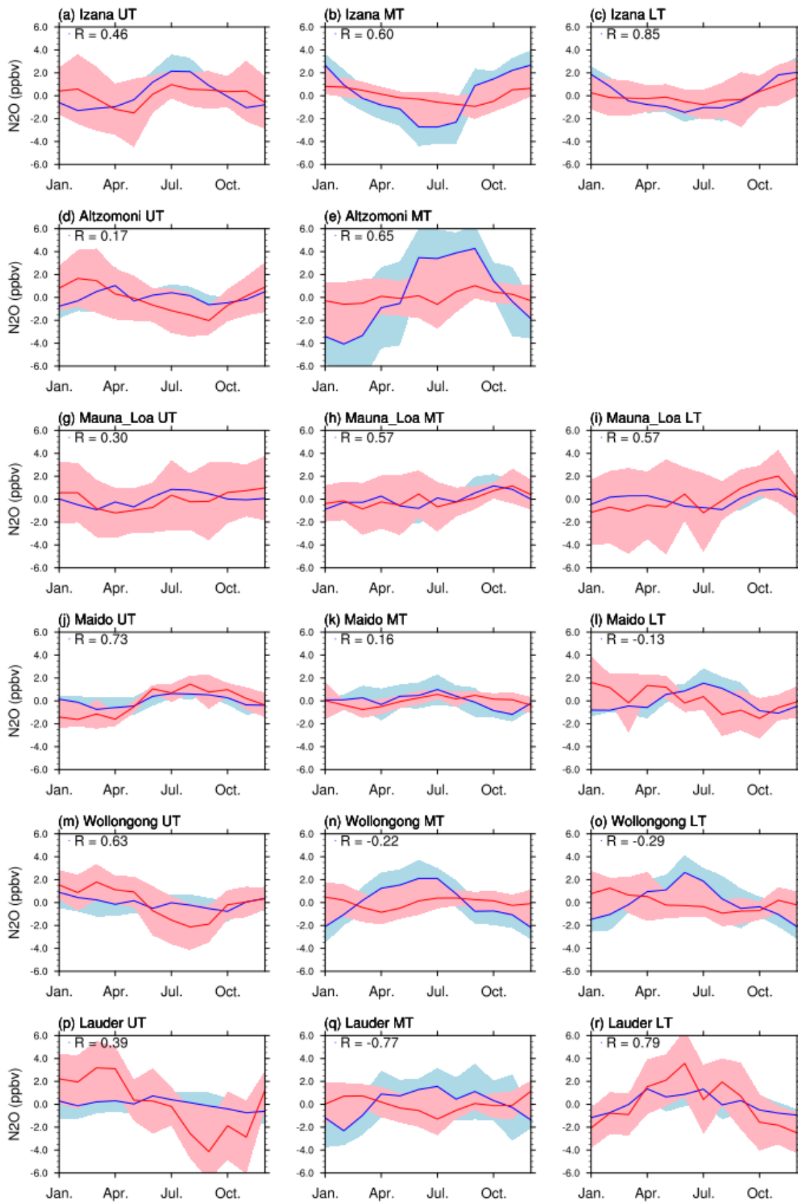
Figure 11. Same as Figure 10 at the 6 tropical and SH stations. There are no data for Alzomoni in the LT (missing panel f) because of the high altitude of the station.
