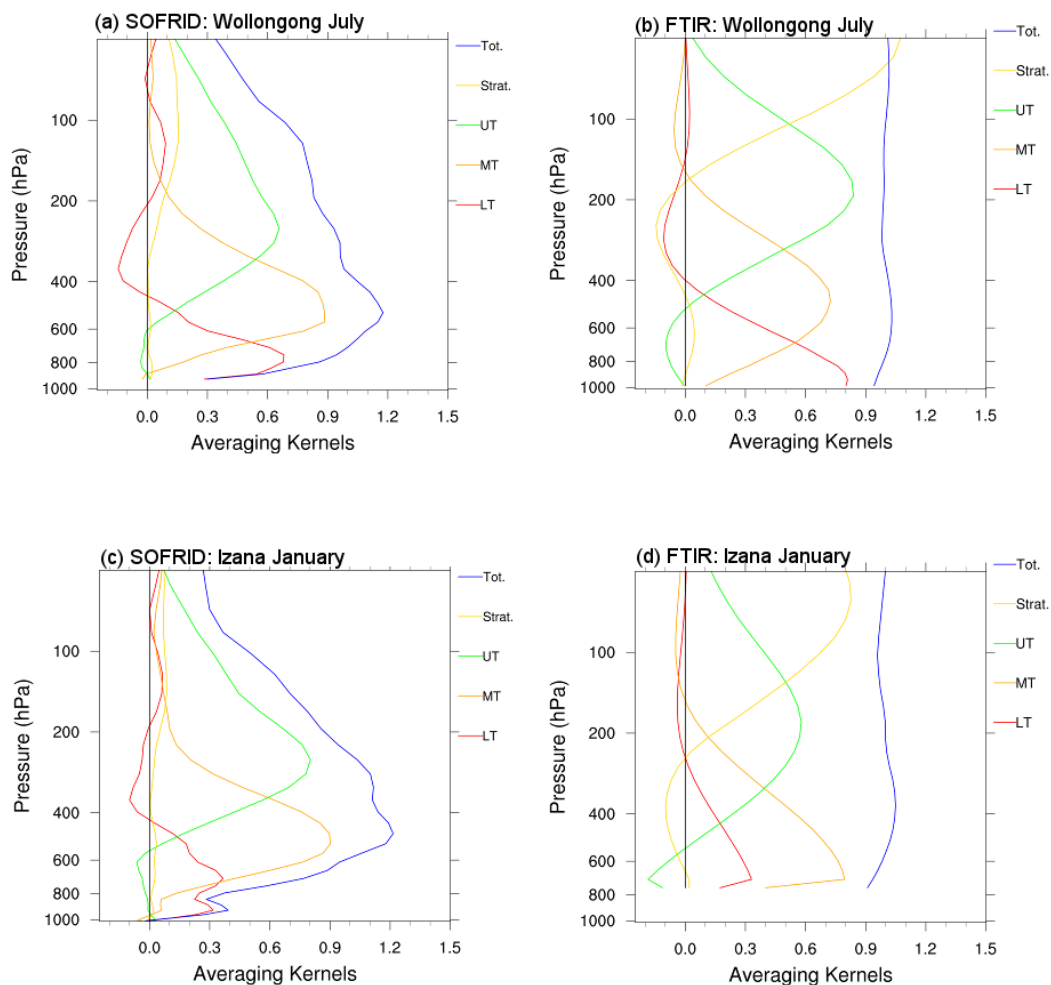
Figure 3. N_2O averaging kernels for (a) IASI in Wollongong in July (b) NDACC in Wollongong in July (c) IASI in Izana in January (d) NDACC in Izana in January. Total Column (Tot), Lower Troposphere (LT, 1013–700 hPa), Middle Troposphere (MT, 700–350 hPa), Upper Troposphere (UT, 350–110 hPa) and Stratosphere (Strat., 100–10 hPa).
