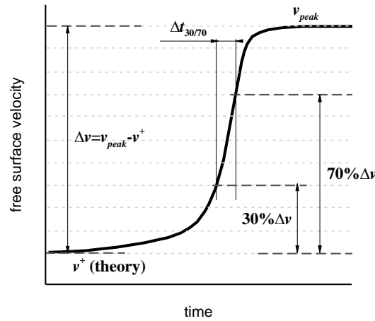
FIGURE 8. Schematic of the definition of the shock layer width according to Eq. (5).
