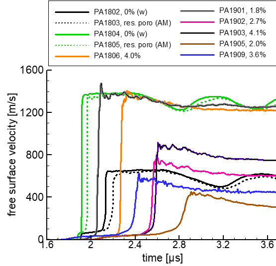
FIGURE 5. Measured free surface velocities in shock experiments on full dense and porous aluminum. The experimental parameters are shown in Table 1.
