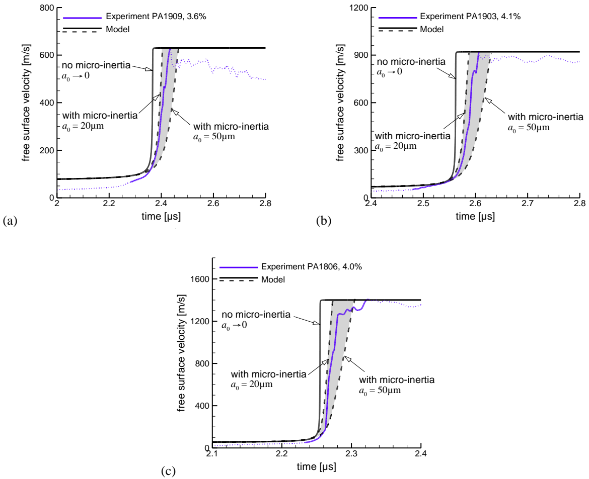
FIGURE 10. Plastic shock profiles for samples with \sim 4\% porosity: comparison between the experimental shock profile and the prediction of the analytical model with no micro-inertia and with micro-inertia. The shaded area marks the plastic shock for a range of pore radii between 20 \mu\text{m} and 50 \mu\text{m} . Experimental curves are represented with solid blue lines in the range [v^+, v_{\text{peak}}] and with thin dashed lines outside this range. The initial porosity considered in the modeling corresponds to those measured in the specimens: (a) 3.6%, (b) 4.1% and (c) 4%.
