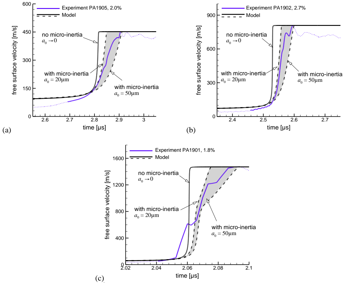
FIGURE 11. Plastic shock profiles for samples of porosity in the range, 1.8%-2.7%: comparison between the experimental shock profiles and the prediction of the analytical model with no micro-inertia and with micro-inertia. The shaded area marks the plastic shock for a range of initial pore radii ( a_0 ) between 20 \mu\text{m} and 50 \mu\text{m} . Experimental curves are represented with solid blue lines in the range [v^+, v_{\text{peak}}] and with thin dashed lines outside this range. The initial porosity considered in the modeling corresponds to those measured in the specimens: (a) 2%, (b) 2.7% and (c) 1.8%.
