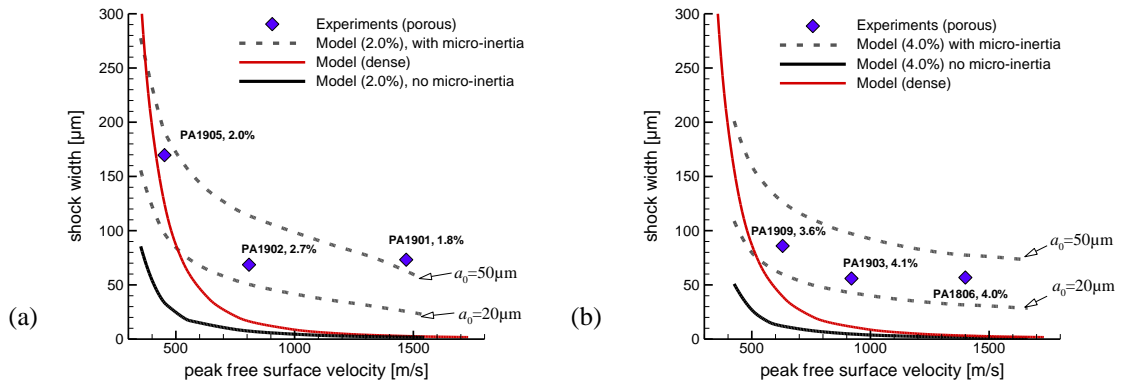
FIGURE 9. Shock width vs. peak free surface velocity for porosity levels of (a) 2% and (b) 4%: dashed lines correspond to theoretical results obtained for two initial void radii, a_0=20 and 50 \mu\text{m} . The solid black line corresponds to the micro-inertia independent case (no effect of pore radius) and the diamond symbols represent the experimental results. The solid red line represents the calculated case of a fully dense material.
