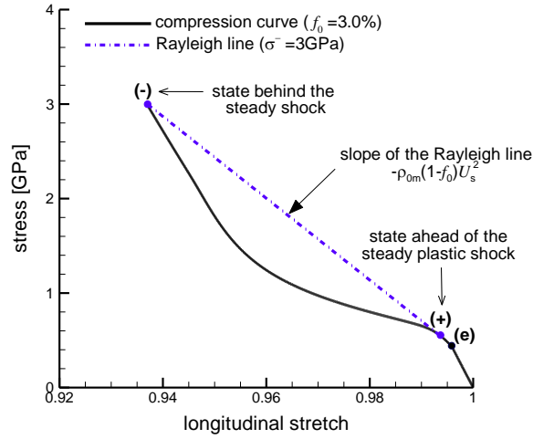
FIGURE 6. Compression curve for porous aluminum ( f_0=3.0\% ) and Rayleigh line defining the shock path from state (+) to state (-) for a shock stress of 3 GPa, see Czarnota et al. [15]. The Rayleigh line, of slope -\rho_{0m}(1-f_0)U_s^2 ( \rho_{0m} being the matrix mass density) is tangent to the compression curve at state (+) and intersects this curve at state (-). From state (e), corresponding to the first plastic yielding, to state (+) ahead of the plastic shock, state variables are varying along the compression curve
