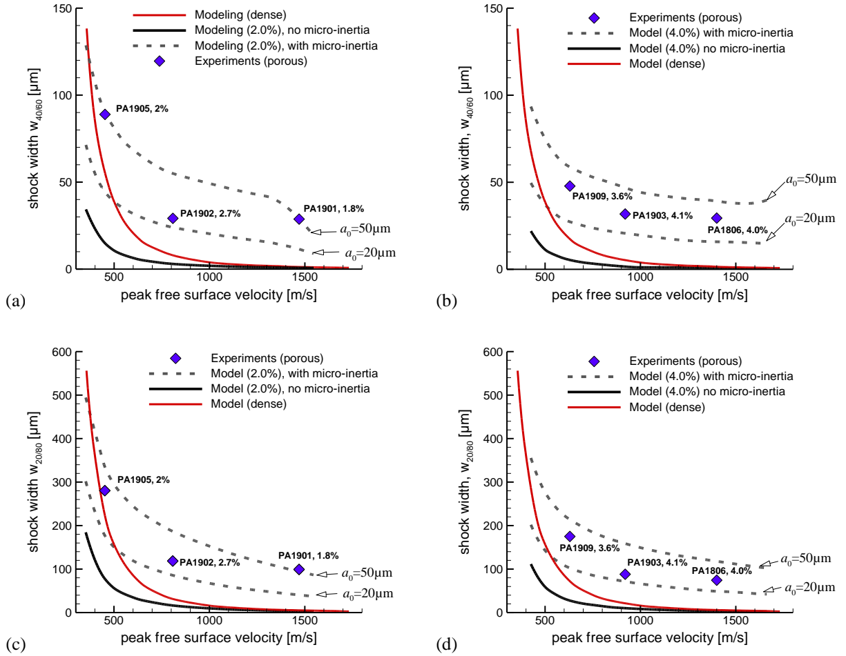
FIGURE 12. Shock layer widths w_{40/60} (a, b) and w_{20/80} (c, d) versus peak free surface velocity v_{peak} for samples of porosity in the range, 1.8%-2.7% (a, c) and of ~4% porosity (b, d). Dashed lines are theoretical results obtained for two initial void radii a_0 = 20 and 50 \mu\text{m} , solid black lines are the micro-inertia independent cases (no effect of pore radius, a_0 ) and the diamond symbols correspond to the experimental results. The solid red lines represent the theoretical predictions for a fully dense material.
