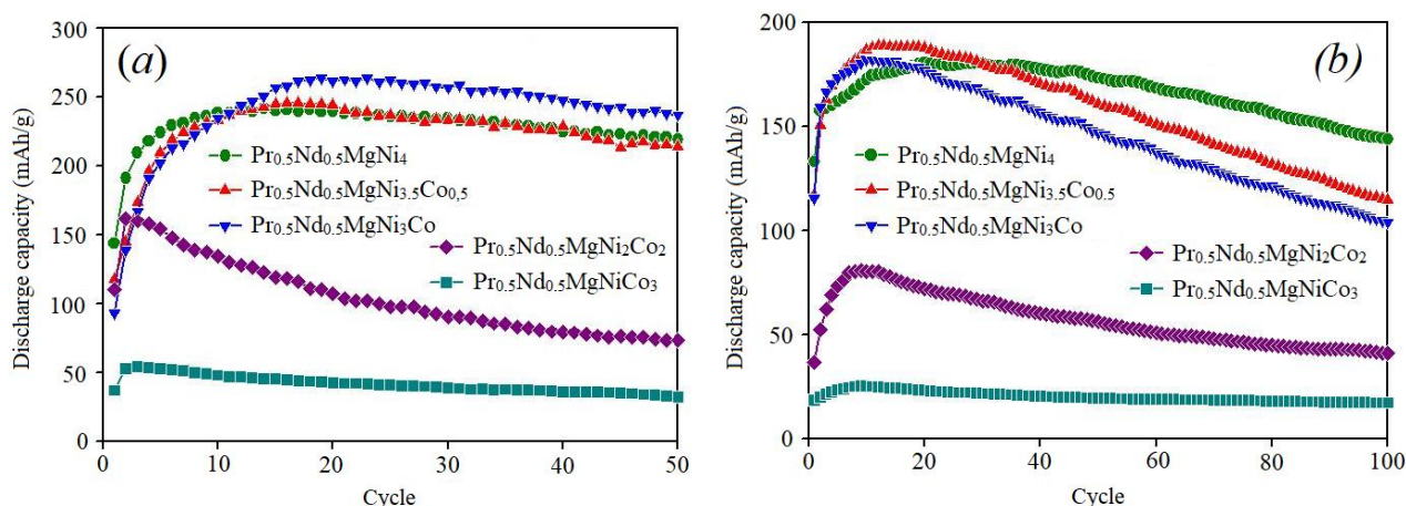
Fig. 6. Cyclic stability of the \text{Pr}_{0.5}\text{Nd}_{0.5}\text{MgNi}_{4-y}\text{Co}_y electrodes. Discharge current density at I = 50 mA/g (a) and I = 200 mA/g (b).
