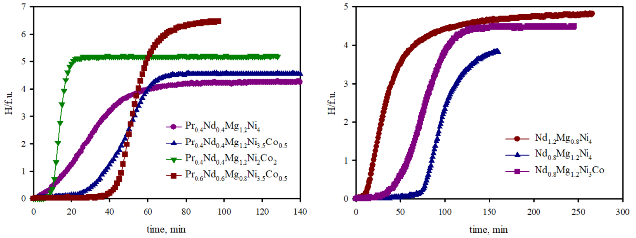
Fig. 3. Curves of first hydrogenation cycle of the selected alloys
