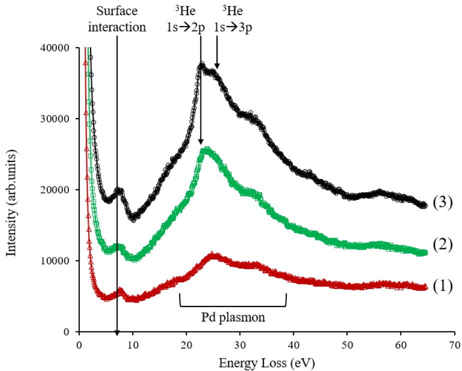
Figure 3 - EELS spectra of Pd matrix (1), Pd matrix + He bubble with 1s \rightarrow 2p transition (2), Pd matrix + He bubble with 1s \rightarrow 2p transition and 1s \rightarrow 3p transition (3) acquired on aged palladium tritide grains with He/Pd=0.23
