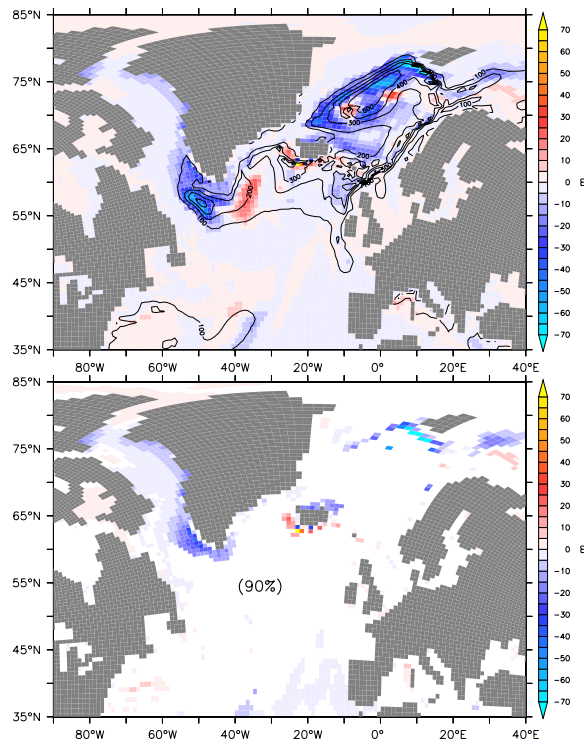
Fig. 9 Shading shows the differences (top figure) and the significant (90%) differences (bottom figure) between Historical and Melting ensemble means for January–February–March mixed-layer depth (in m) averaged over the period 1920–2014. Contour lines are the mean state of the Historical ensemble mean over 1920–2014
