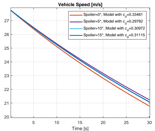
Fig. 2. Deceleration experiments for different spoiler positions with vehicle mass=1950kg
