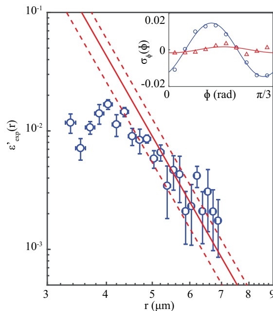
Fig. 5 Experimental determination of the azimuthal interaction. Evolution of the amplitude of oscillations shown in Fig.4F, as a function of the distance decaying as \propto 1/r^7 . Red solid and dashed lines are the mean value and its extrema, respectively, as predicted by the numerical simulation in the absence of adjustable parameter (see main text). It shows an excellent agreement with the experimental data. Inset: Profiles of Fig.4F, at distances of 4 (blue circles) and 6 \mu\text{m} (red triangles) from the center of the rotor. Solid lines are fits using a sinusoidal function. It confirms diffusiophoresis as the source of interaction.
