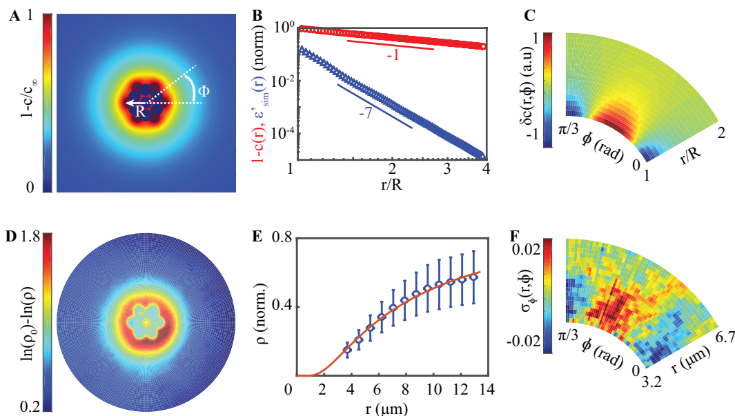
Fig. 4 Anisotropic and diffusiophoretic interactions. A), B), C) are simulations and D), E), F) are experiments. A) Numerical mapping of the (normalized) concentration field around a rotor of radius R , situated above an impermeable interface. At fixed distance, the concentration profile is periodically modulated by the presence of the haematite. B) Evolution of the radial concentration profile (after azimuthal average, red circles), following a \propto 1/r decay. The azimuthal profile follows a sinusoidal variation in the interval [0; \pi/3] with decaying amplitude \varepsilon'_{\text{sim}} \propto 1/r^7 (blue triangles, see main text). C) Mapping of the azimuthal variations after subtracting the radial dependency (see main text). D) Experimental observation of the interaction profile between a rotor and 20 nm fluorescent beads using HILO microscopy, in the reference frame of the rotor. The data closely resemble A). E) The radial density profile of the fluorescent beads (blue circles) follows eq.(2) (red line), with \alpha = 120 \mu\text{m}^3/\text{s} . F) Experimental mapping \sigma_\phi of the azimuthal interactions after removal of the radial contribution (see main text). A periodic modulation is visible, with the higher repulsion near the haematite.
