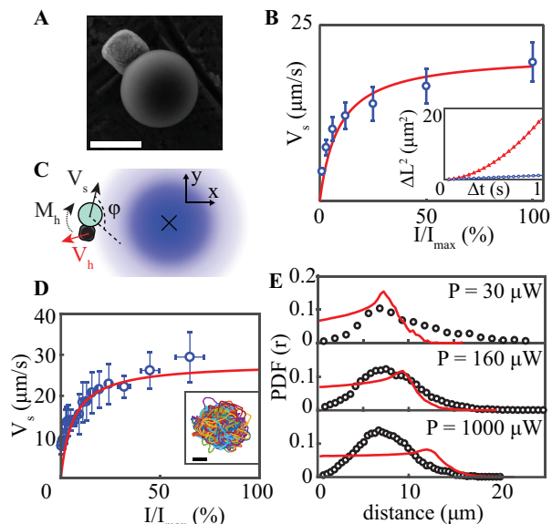
Fig. 2 A phototactic microswimmer. A) SEM image of the phototactic swimmer, which consists of a haematite particle extruded from a colloidal bead. Scale bar is 1 \mu\text{m} . B) The swimmer exhibits persistent random walk under homogeneous illumination with a velocity (blue circles) tuned by the light intensity ( I_{\text{max}} = 550 \text{ nW}/\mu\text{m}^2 ). The red line is a fit using eq.(5), and I_{\text{sat}} = 50 \text{ nW}/\mu\text{m}^2 . Inset shows the Mean Square Displacement (\Delta L)^2 of swimmers at equilibrium (no illumination, blue circles) and under illumination (red triangles), at I/I_{\text{max}} = 10^{-2} . Solid lines are fits with eq.(4). For I = 0 , we get D_s = 0.3 \pm 0.1 \mu\text{m}^2/\text{s} . C) Scheme of the phototactic mechanism. As the haematite is phoretically repelled from higher intensities of light, it reorients the swimmer along the gradient, inducing an effective torque \mathbf{M}_h . The blue spot represents the laser used in the experiment and the notations are the ones from main text. D) Evolution of the speed V_s(I) of individual swimmers under the same excitation profile and intensities as for the haematite in section 2, ( I_{\text{max}} = 1200 \text{ nW}/\mu\text{m}^2 ). The solid line follows eq.(5), with V_{\text{sat}} = 24 \mu\text{m}/\text{s} and I_{\text{sat}} = 75 \text{ nW}/\mu\text{m}^2 . Inset shows the trajectories of the swimmers around the laser spot. Scale bar is 5 \mu\text{m} . E) Density of Probability of Presence of the swimmers (PDF) at distance r from the center for 3 different excitation powers (black circles). It shows a reasonable agreement with our simulations of ABP, notably the range of the trajectories, without any adjustable parameter (solid red lines, see main text).
