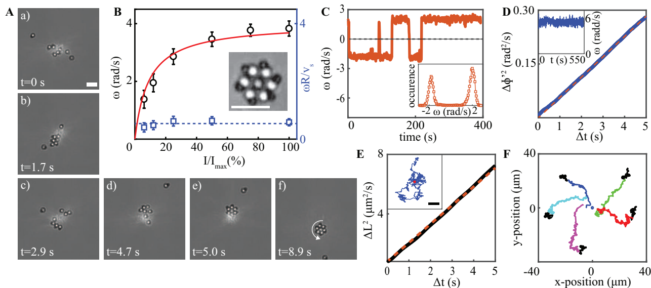
Fig. 3 Formation mechanism and properties of the rotor. A) Snapshots of a movie showing the assembly of a rotor around a single laser spot. In (a) the swimmers travel around the laser spot, until they assemble, (b) and form a transient structure that breaks, (c). The swimmers collide again, (d) and form a stable rotor (e), which is sustained under illumination after removing the gradient (f). B) The angular speed of the rotor is tuned by the light intensity. The solid red line is a fit with eq.(5), using the same saturation intensity as for the swimmers alone. The angular speed reflects the speed of the swimmers (blue squares). Inset: magnified image of a rotor, where the orientation of the swimmers is visible. C) At low angular speeds ( \omega < 3 rad/s), the rotor can flip its direction of rotation. Inset: distribution of speeds for a rotor during a \sim 10 min experiment. The two peaks are situated at -1.8 and 1.9 rad/s, showing the symmetry of the dynamics. D) At higher speeds, the motion is persistent and the angular fluctuations can be extracted (blue line). Dashed red line shows a linear fit using eq.(8), and gives D_\Phi = 0.03 \pm 0.01 rad 2 /s. Inset: speed of a fast rotor ( \omega \sim 6 rad/s) over 10 min. E) Experimental MSD (black curve) of free-to-move rotors, and linear fit (red dashed line), giving D_R = 0.4 \pm 0.1 \mu\text{m}^2/\text{s} . Inset: trajectory of the center of mass of rotor optically trapped with a red laser (red) and free to diffuse (blue) (see main text and Methods). F) Migration of rotors in light gradient, for 5 different experiments. The rotors first exhibit a diffusive motion in homogeneous light, (black curves, 15 s for each experiment) but migrate towards the bright spot (colored curves) of a focused laser light (circle at the center). Typical time for migration is 10 – 30 s. All scale bars are 5 \mu\text{m} .
