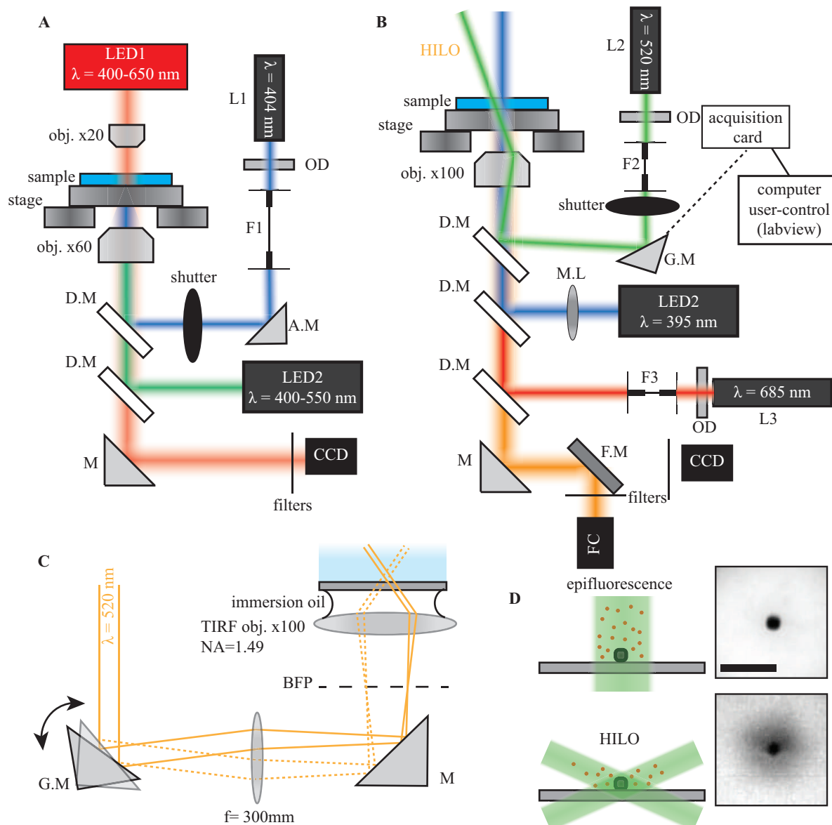
Fig. 6 Experimental setups. See main text for full description. A) Experimental setup used for rotor creation. B) Highly Inclined Laminated Optical sheets (HILO) microscopy setup used for imaging the concentration profile around a rotor. C) Detailed scheme showing the light path for HILO microscopy. The laser is focused at the back focal plane of a high-NA objective. Shifting the position of the laser with respect to the center of the entrance pupil results in inclined, output light beams. D) Top : In standard epifluorescence microscopy, background fluorescence is high because of strong illumination of the planes above the focal plane. Bottom : In HILO microscopy, only a small slice ( \sim few microns) above the focal plane is shined, lowering the background fluorescence. The images on the right show the fluorescence profile of beads around a haematite in epifluorescence (top), compared to HILO (bottom). Scale bar is 5 \mu\text{m} . The symbols used are : L1, L2, L3 : Laser sources; DM : Dichroic Mirror; GM : 2-axis Galvanometric Mirror; F1 : Multimode Fiber; F2, F3 : Single Mode fibers; OD : Optical Densities; FM : Flip Mirror; AM : Adjustable Mirror ML : Movable Lens; FC : Fluorescence Camera; CCD : Charged-Coupled-Device camera; M : Mirror. For better clarity, we do not represent optical lenses.
