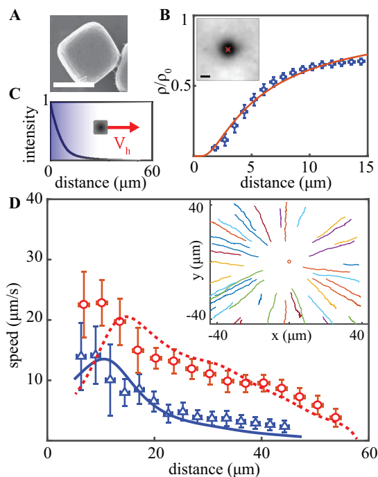
Fig. 1 Response of haematite under illumination. A) SEM image of a haematite particle. Scale bar is 500 nm. B) Isotropic phoretic repulsion of 20 nm fluorescent beads around a haematite particle tethered on the surface of a capillary, under uniform blue ( \lambda = 395 \text{ nm} ) excitation. The density of fluorescent beads (blue circles) decays when approaching the haematite particle, and follows eq.(2) (red line), with \alpha = 64 \mu\text{m}^3/\text{s} . Inset: repulsion of FB in the XY plane. The red cross locates the haematite particle (scale bar 5 \mu\text{m} ). C) Isotropic intensity profile generated with a slightly defocused blue laser spot ( \lambda = 404 \text{ nm} ), after azimuthal averaging, used for analyzing the response of haematite in a gradient of light. An asymmetric reaction rate occurs at the surface of the haematite, triggering its motion at speed V_h by self-diffusiophoresis. D) Recorded speeds of haematite particles in the intensity gradient shown in C), at excitation power of P=0.16 \text{ mW} (blue triangles) and P=1 \text{ mW} (red circles). The velocity is adjusted with eq.(3) (solid blue line and dashed red line) from the measured intensity profile and using constant saturation intensity (see main text). Inset: trajectories of individual haematite particles, isotropically repelled from the laser spot (red dot), at P=1 \text{ mW} .
