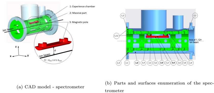
Figure 6: Spectrometer: CAD model and enumeration of parts and surfaces.
