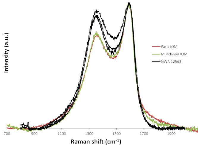
709 710 Fig. 21. Raman spectra of the NWA 12563 chondrite compared to spectra from CM2 chondrites.
