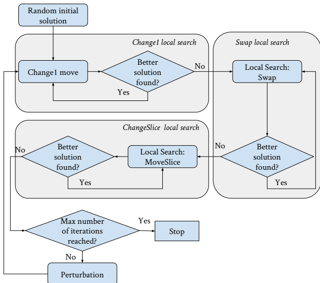
Fig. 3: VNS algorithm as implemented in MorpheuS.
