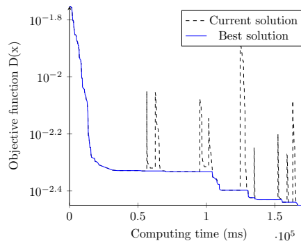
Fig. 5: Evolution of objective function values over time during a run of the VNS algorithm.
