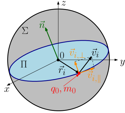
FIG. 2. Instantaneous decomposition of the charge velocity \vec{v}_i in the two components tangent \vec{v}_{i,\parallel} and perpendicular \vec{v}_{i,\perp} to the instantaneous position of the dipole circle. The perpendicular component is crucial for the introduction of the damping force. While \Pi represents the dipole plane, \Sigma is the sphere circumscribed to the dipole.
