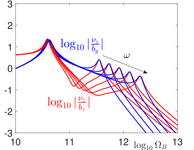
FIG. 4. Frequency response of the system with a varying value of the intrinsic frequency \omega . We adopted the parameters \gamma = 1.76 \times 10^{11} \text{s}^{-1} \text{T}^{-1} , B = 0.25 \text{T} , \alpha = 0.1 and \omega = 1.6 \times 10^{11}, 2.5 \times 10^{11}, 4 \times 10^{11}, 6.3 \times 10^{11}, 1 \times 10^{12} \text{s}^{-1} . The arrow indicates the increasing values of \omega .
