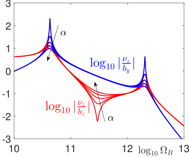
FIG. 5. Frequency response of the system with a varying value of the damping factor \alpha . We adopted the parameters \gamma = 1.76 \times 10^{11} \text{s}^{-1} \text{T}^{-1} , B = 0.25 \text{T} , \alpha = 0.01, 0.06, 0.11, 0.16, 0.21 and \omega = 1 \times 10^{12} \text{s}^{-1} . The arrow indicates the increasing values of \alpha .
