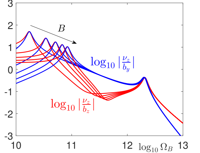
FIG. 3. Frequency response of the system with a varying value of the applied magnetic induction B . We adopted the parameters \gamma = 1.76 \times 10^{11} \text{s}^{-1} \text{T}^{-1} , B = 0.1, 0.2, 0.3, 0.4, 0.5 \text{T} , \alpha = 0.1 and \omega = 1 \times 10^{12} \text{s}^{-1} . The arrow indicates the increasing values of B .
