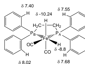
Figure 2. Representation of the structure for \text{Fe}(\text{CO})_2(\text{dppe})(\text{H})_2 2 illustrating key NMR features.
