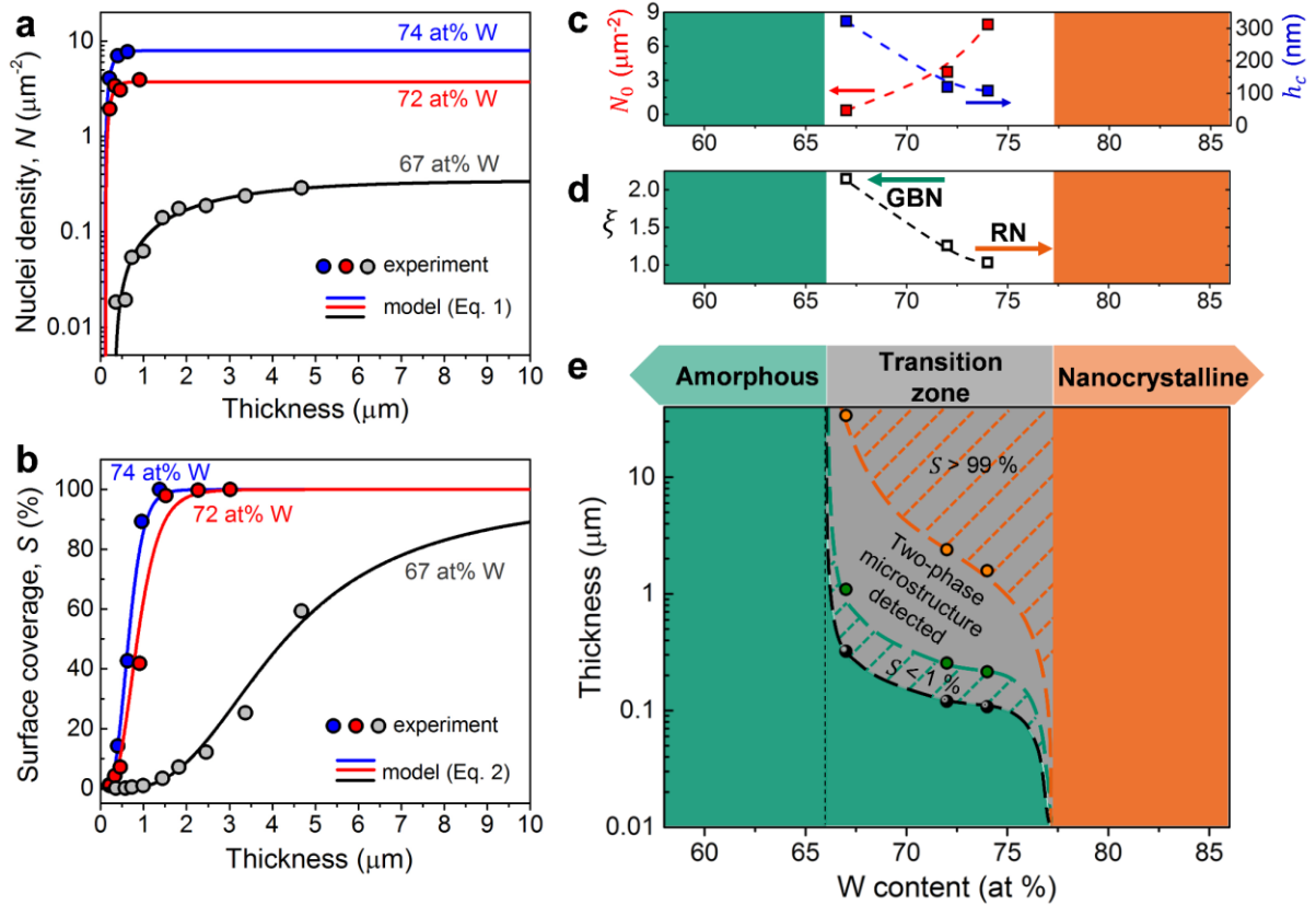
Figure 4. Thickness-composition metastable Zr-W phase diagram. (a) Evolution of the density of nanocrystalline nuclei and (b) surface coverage by the nanocrystalline phase with the increase of the film thickness for the three compositions studied. The dots represent the experimental data. In (a) the lines follow Equation 1. In (b) the lines follow Equation 2. (c) Values of N_0 (red squares) and h_c (blue squares) obtained from the fitting of Equation 1 to the data corresponding to the density of nanocrystalline nuclei. (d) Values of \xi obtained from the fitting of Equation 2 to the data corresponding to the surface coverage by the nanocrystalline phase. RN and GBN indicate random nucleation and grain boundaries nucleation, respectively. (e) Depending on composition, the structure of the films can be single-phased amorphous (green zone), single-phased nanocrystalline (orange zone) or bi-phased in the transition zone (gray zone). In this domain are shown the values of the critical thickness h_c (black points) and the thickness at which the surface coverage, S , is lower than 1% (green points) and higher than 99% (orange points). The last two thicknesses were calculated from extrapolation of Equation 2.
