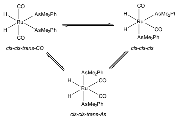
Scheme 2: Observed isomers of Ru(AsMe 2 Ph) 2 (CO) 2 (H) 2 .
