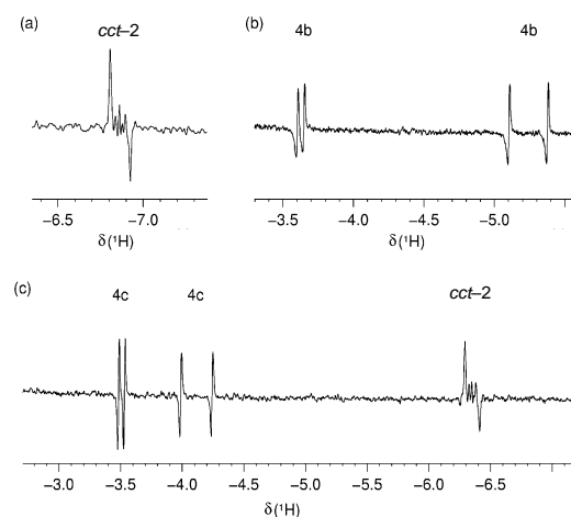
Figure 1. Selected regions of NMR spectra obtained at 255 K during the reaction between \text{Ru}(\text{CO})_3(\text{PPh}_3)_2 and p\text{-H}_2 with concurrent laser irradiation: (a) 32 transient ^1\text{H} spectrum of \text{Ru}(\text{CO})_2(\text{PPh}_3)_2(\text{H})_2 , cct-2 , in toluene- d_8 ; (b) ^1\text{H} spectrum illustrating the hydride resonances of \text{Ru}(\text{CO})_2(\text{PPh}_3)(\text{THF-}d_8)(\text{H})_2 4b (c) ^1\text{H} spectrum in pyridine- d_5 showing \text{Ru}(\text{CO})_2(\text{PPh}_3)(\text{pyridine-}d_5)(\text{H})_2 4c .
