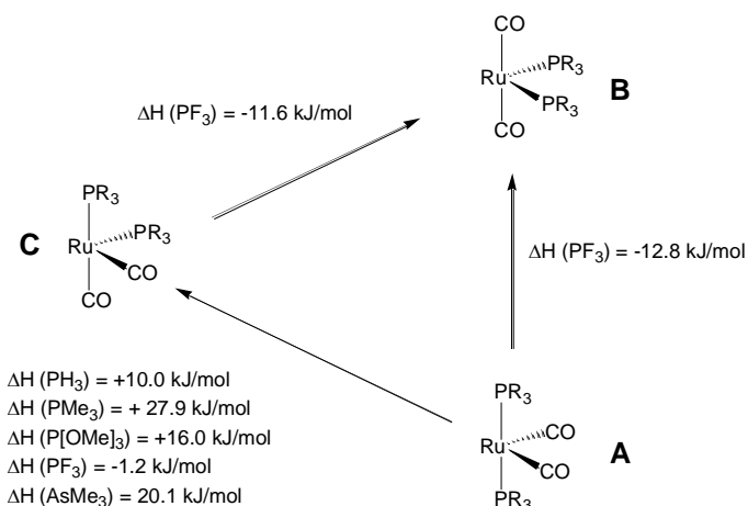
Figure 6. Relative energies calculated for the 16-electron intermediates.
