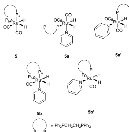
Figure 5. Products formed from the photolysis of Ru(CO) 3 (dppe) with 3 atm of p -H 2 in pyridine- d 5
