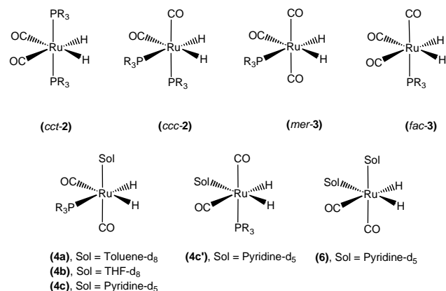
Figure 2. Proposed structures for compounds 2–4 and 6 identified in this study, where R = Ph, Me, Cy or p -tolyl.
