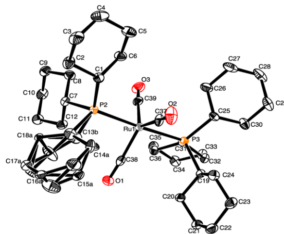
Figure 3. Crystal structure of \text{Ru}(\text{CO})_3(\text{PCy}_3)_2 .
