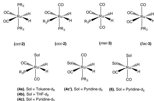
Figure 2. Proposed structures for compounds 2–4 and 6 identified in this study, where R = Ph, Me, Cy or p -tolyl.
