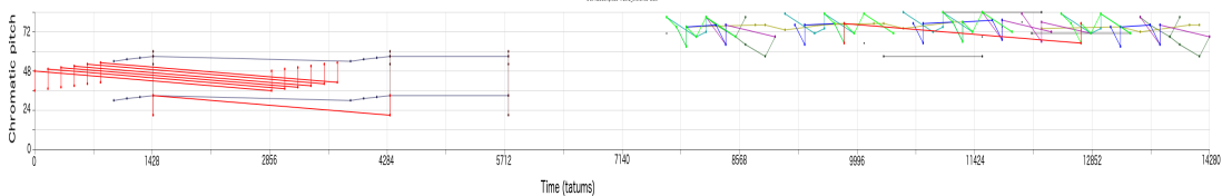
(c) Pattern set C: SIATECCompress (no restrictions on the pattern length), compression ratio: 1.58, number of TECs: 11. Each TEC is represented with a different color.
