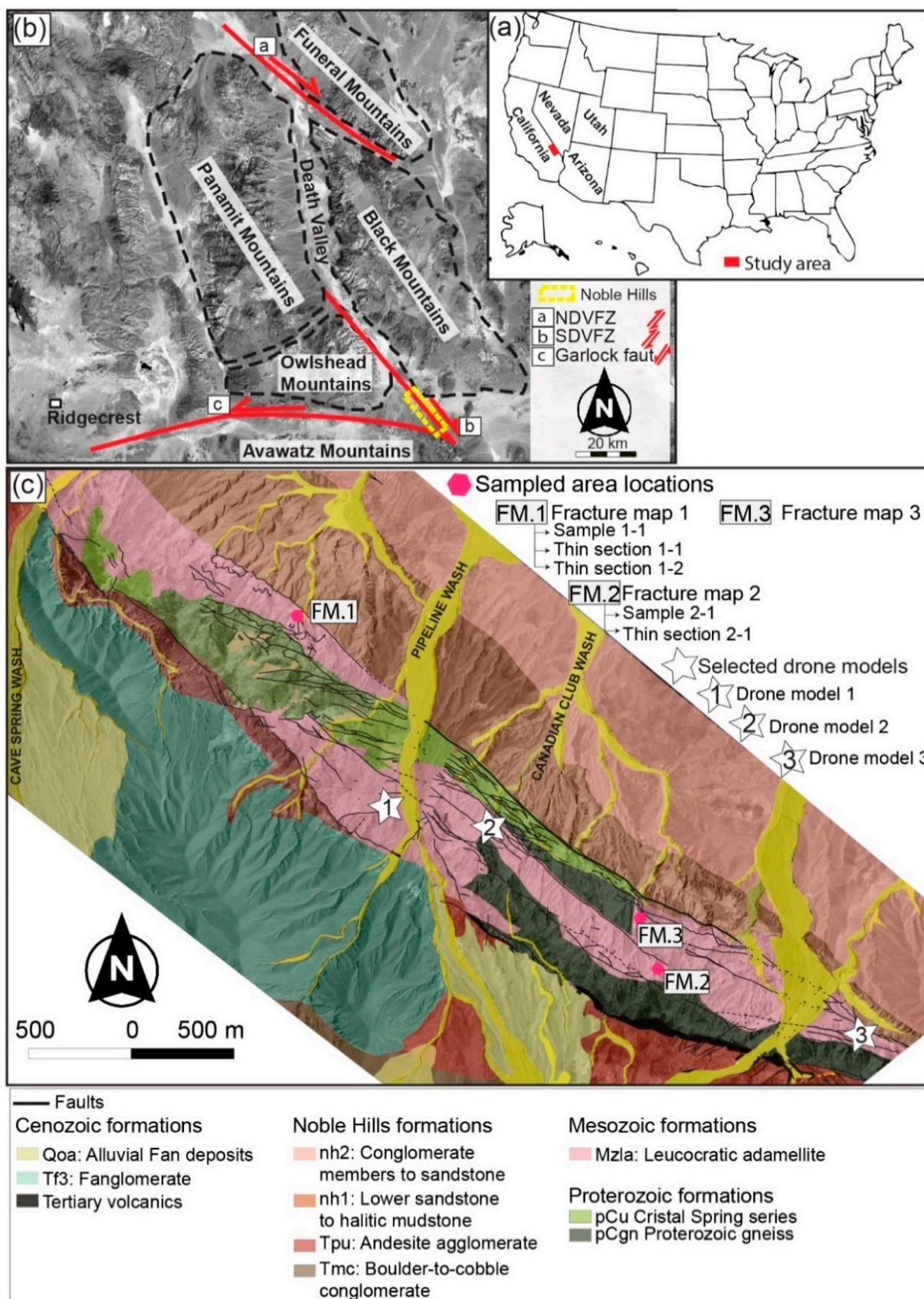
Figure 1. (a,b) Location and geological setting of DV, NDVZFZ: Northern Death Valley Fault Zone, SDVZFZ: Southern Death Valley Fault Zone; (c) Structural scheme of the NH range built using high-resolution digital mapping techniques modified after [37,39]. Additional digitized fractures were performed using orthophotos. The aerial picture in (b) was extracted from Google Earth®. The samples location was reported in the structural scheme. FM: fracture map.
