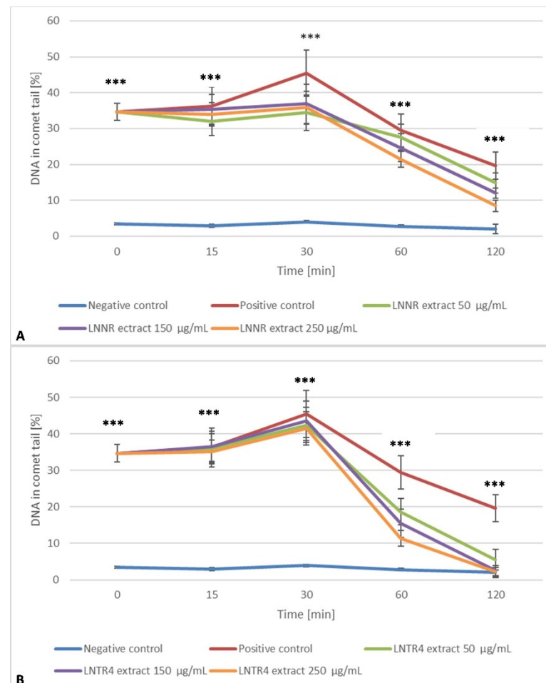
Figure 8. LNNR (A) and LNTR4 (B) root extracts showed DNA damage in human umbilical vein endothelial cells (HUVEC), treated with 75 µM hydrogen peroxide for 10 min at 4 °C (time 0), then incubated with both extracts within the range of concentrations from 50 to 250 µg/mL and measured for 15, 30, 60, and 120 min. Negative control is the lack of damage agents. Positive controls were treated with hydrogen peroxide alone. The values were measured as the mean percentage of DNA in the comet's tail \pm SD in the alkaline version of the comet assay. The tail DNA fraction was determined for 50 comets in each trial. *** p < 0.001 comparison control vs. extracts with H 2 O 2 .
