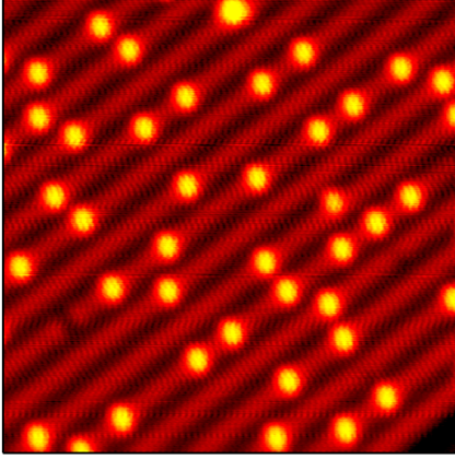
FIG. 5. (Color online) (a) 19.7 \times 19.7 \text{ nm}^2 constant current mode STM image of a 0.01 ML K-doped IrTe 2 sample, V_{\text{bias}} = -200 \text{ mV} , I = 0.2 \text{ nA} .
