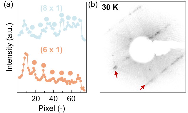
FIG. 6. (a) Lines profiles of LEED images shown in (b). (b) LEED image from a 0.13 ML K doped crystal of IrTe 2 in the (8 \times 1) and (6 \times 1) phases at 30 K. All images were obtained using 64 eV electron energy.
