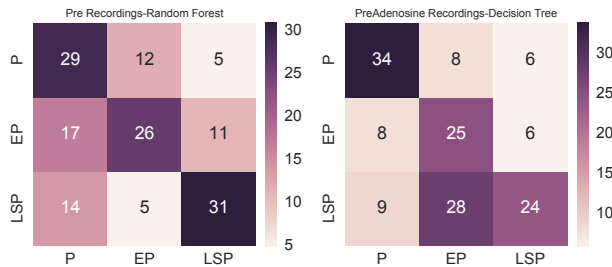
Figure 2. Confusion matrices for the best model for Pre and PreAdenosine (P=PAF, EP=E-PeAF, LSP=LS-PeAF). The number in each box gives the number of TQ segments.
