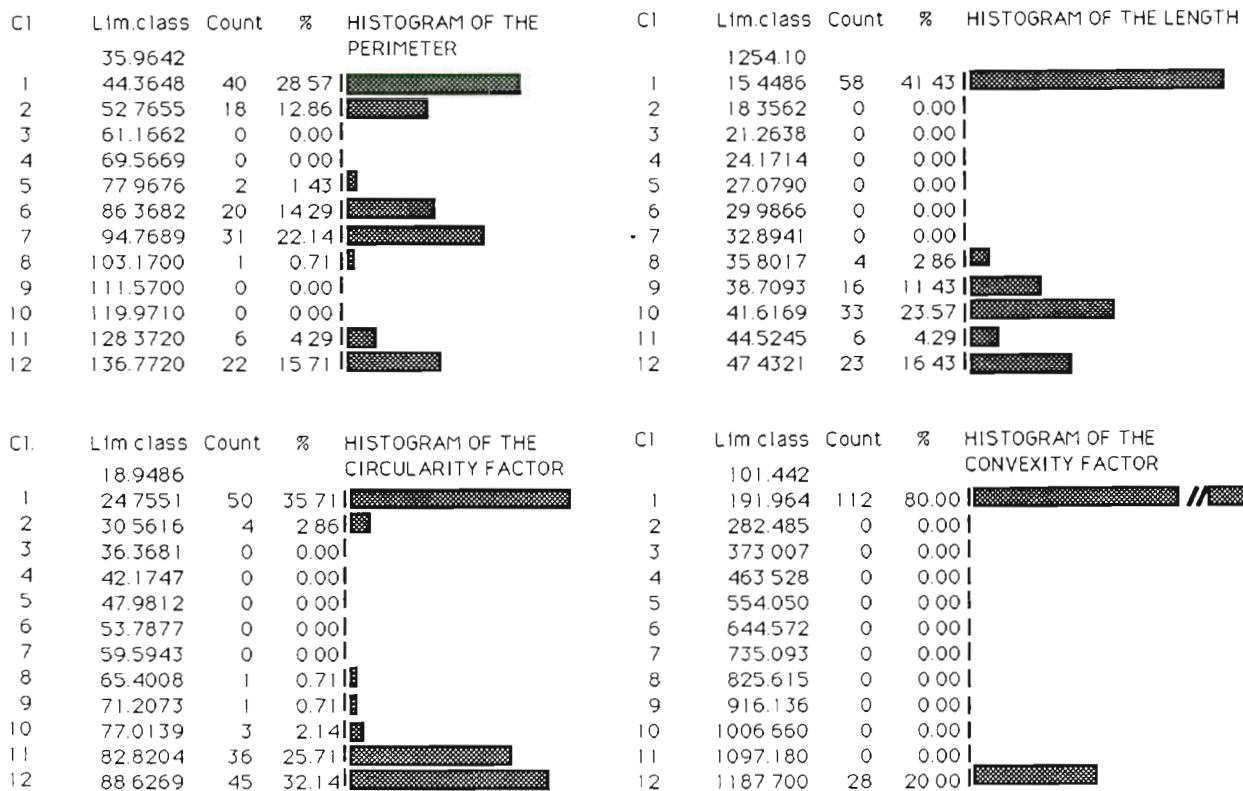
Fig. 5. Results printout of an automatic analysis of the 3 algae samples. Notice the trimodal distribution of the perimeter measurements histogram differentiating between the 3 algal species
