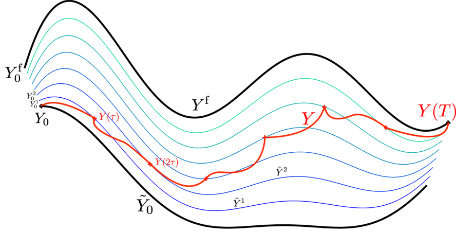
FIGURE 2. Schematic representation of the staircase method used for the proof of Theorem 2.8.
