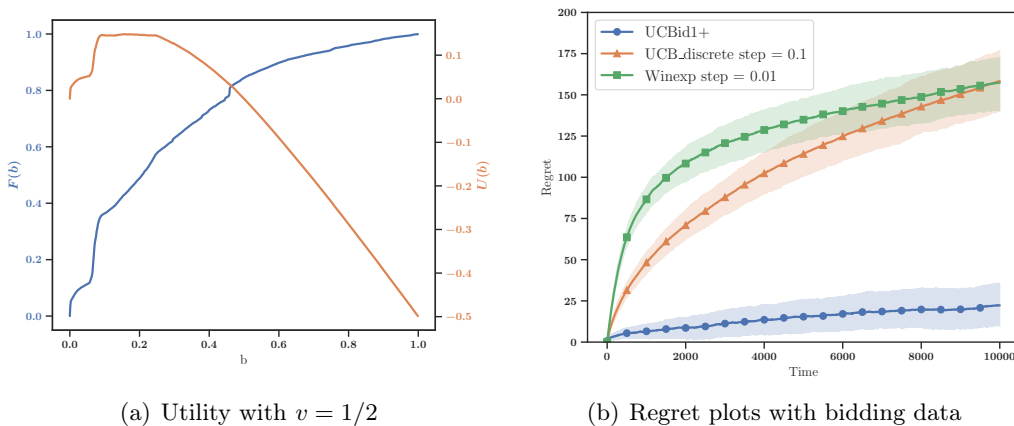
Figure 7: Experiment with real bidding data
