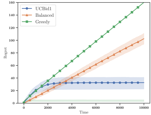
(b) Regret plots under the second instance of the problem
