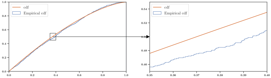
Figure 2: Local behavior of the empirical CDF
