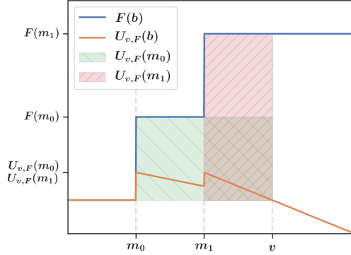
Figure 1: An example with two maximizers
