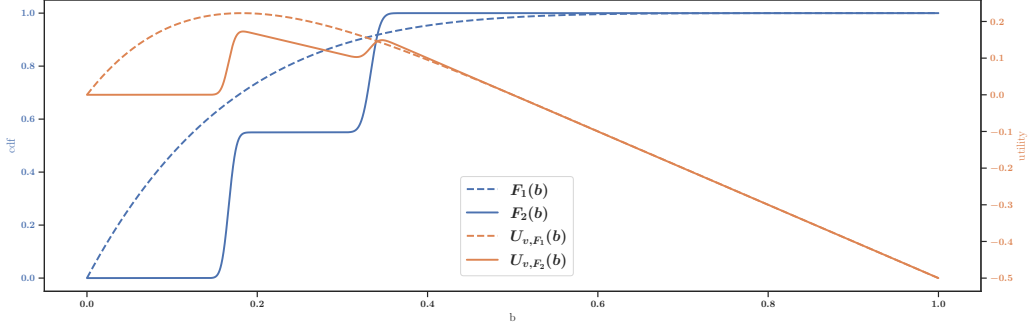
Figure 3: Two choices of F ; associated utilities for v = 1/2 .
