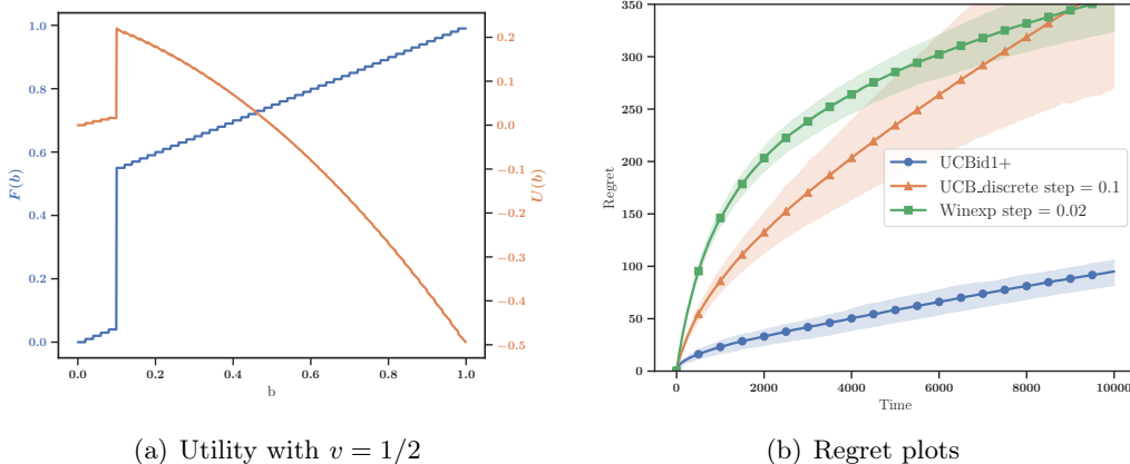
Figure 6: An example with discrete bids
