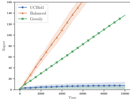
(a) Regret plots under the first instance of the problem
