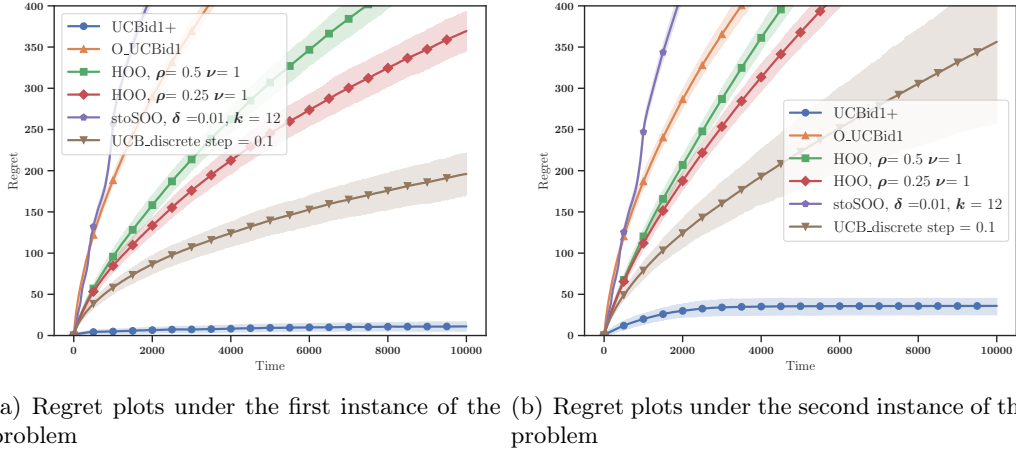
Figure 5: Regret plots for unknown F
