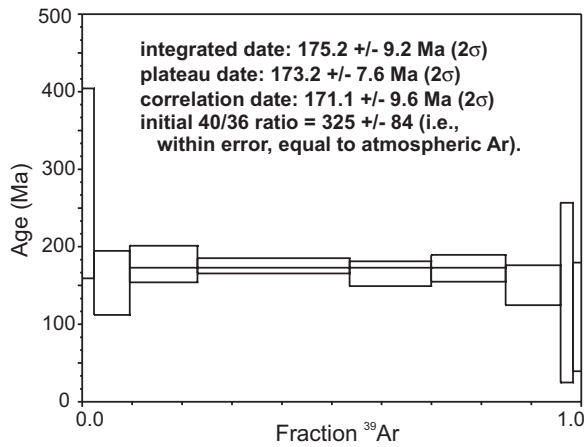
Figure 6. Step heating ^{40}\text{Ar}/^{39}\text{Ar} age spectrum for French Range blueschist sample MMI96-4Bwr.
