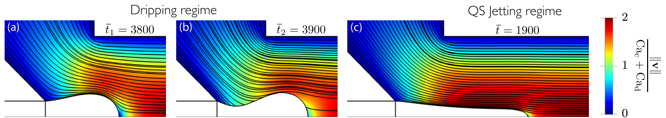
Figure 9. Axisymmetric simulations in transient using couple 1 (see Table 1) and Ca_d = 8 \cdot 10^{-5} (QS limit). The flow field is represented by streamlines and rescaled velocity norm \|v_c\|/(Ca_c + Ca_d) as color code. The timescale is R_n \mu_c / \gamma = 7 \mu s . (a,b) Dripping regime with Ca_c = 0.1 for a time before (a) and after (b) the folding bifurcation; (c) QS-jetting regime for Ca_c = 0.3 > Ca_c^* (see section Inviscid droplets for details).
