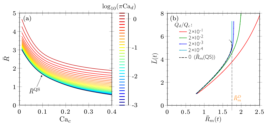
Figure 8. (a) Influence of the Ca_d on the generated drop radius as a function of Ca_c computed in transient considering couple 1 (see Table 1); \bar{R}^{QS} in black line corresponds to Ca_d = 4 \times 10^{-6} \pi^{-1} , i.e. the quasi-static limit. (b) Transient evolution of the meniscus length \bar{L} as a function of the meniscus equivalent radius \bar{R}_m for different values of \bar{Q} = Q_d/Q_c and Ca_c = 0.1 , considering couple 1 (see Table 1). The equivalent radius of the meniscus calculated with quasi-static simulations is plotted in black dashed line.
