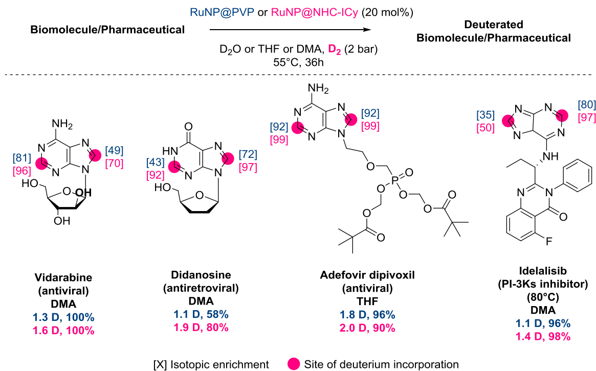
Figure XX. Deuterium labelling of pharmaceuticals. In blue, isotopic enrichment obtained with RuNP@PVP and in pink with RuNP@NHC.
