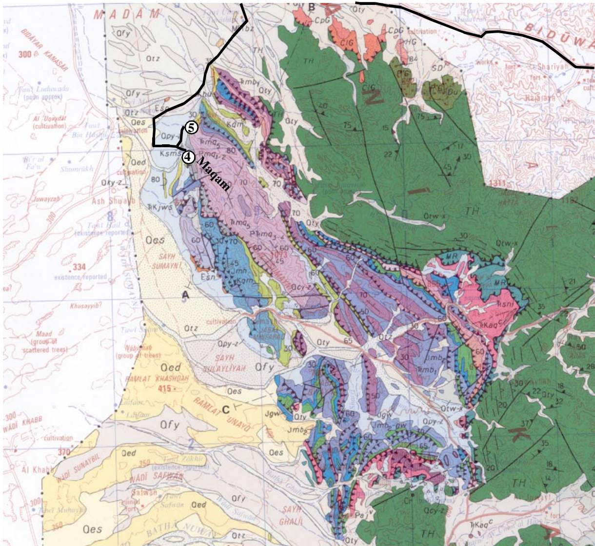
Figure 21- Geological map of the Sumeini area (Map Buraymi, Le Metour et al., 1992).
