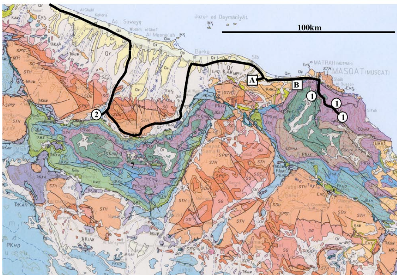
Fig. 4: Geological Map of the Field excursion B01, with the main stops (1-2) and places of overnight (A, B). Map from Le Métour et al., (1993a)
