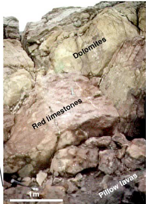
Figure 15- The Rustaq section 1 outcrop.. Details of the sedimentary cover above the pillow lavas.
