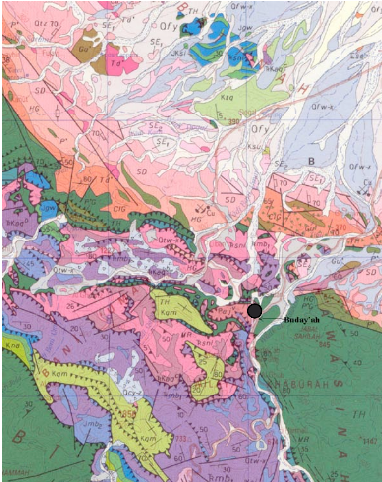
Fig. 11- Geological map of Buday'ah area (Map Ibri, Béchenec et al., 1992c)
