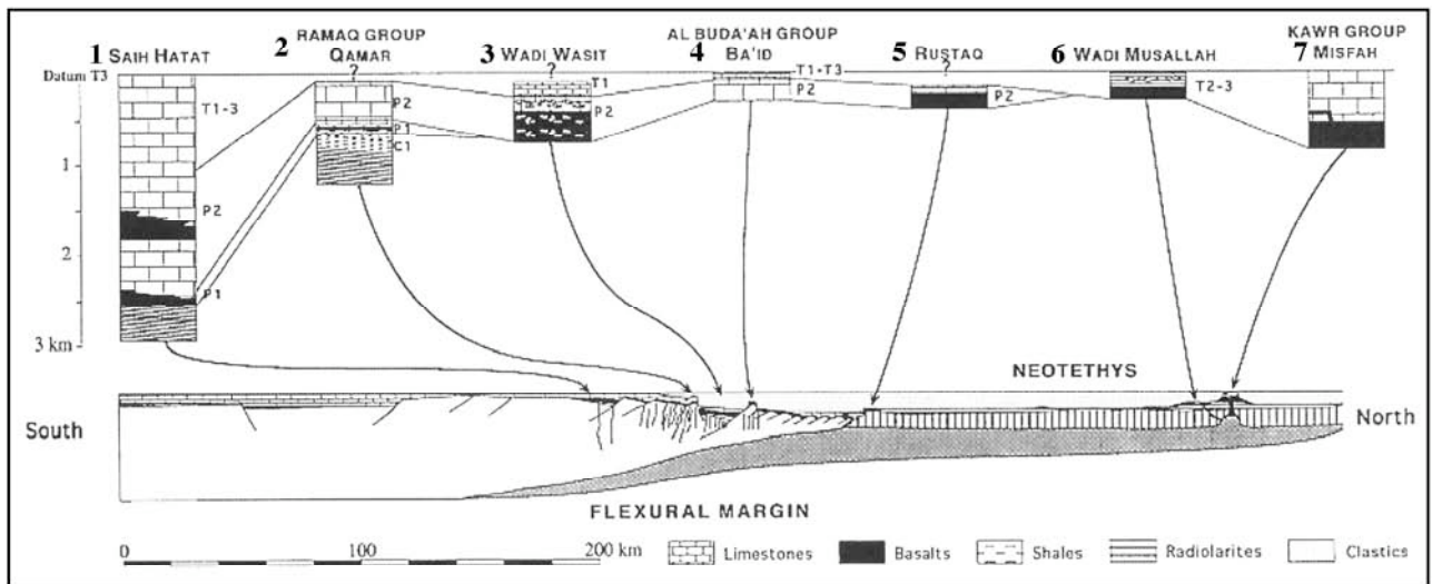
Fig. 6 -Oman margin in the late Triassic, from proximal (1) to distal (7) (after Pillevuitt et al., 1997).
