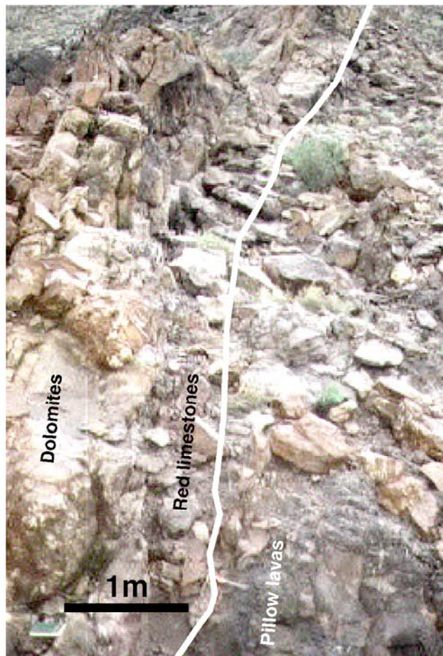
Figure 14- The Rustaq section 1 outcrop. View of the contact between the pillow lavas and the sedimentary cover.
