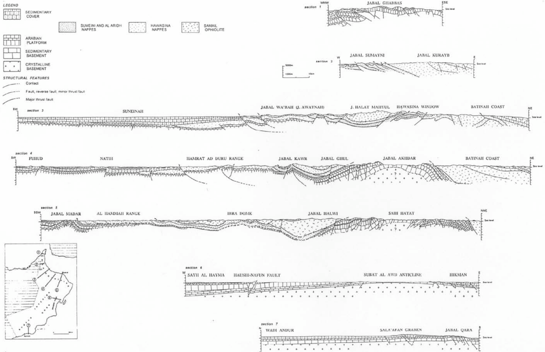
Fig. 2- Structural cross-sections from the N to the S of Oman (from Le Métour et al., 1995)
