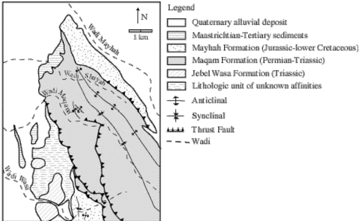
Figure- 23 Simplified geological map of Sumeini Area. (After Watts & Garrison, 1986).
