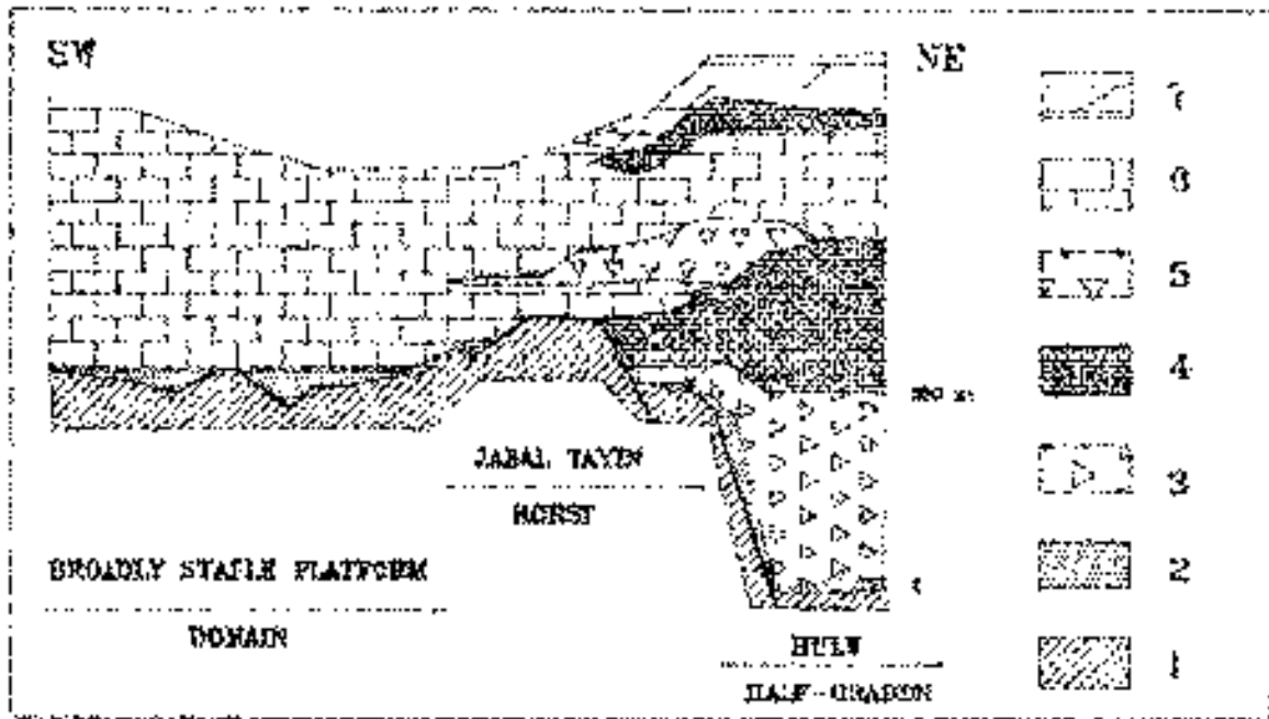
Figure 9 – Paleogeographical diagram showing the distribution of various lithologic facies on the Permian platform. 1: Pre-Permian series; 2: conglomerate, sandstone and siltstone; 3: rhyodacitic tuffite; 4: external platform carbonate; 5: trachy-andesitic and basaltic lava; 6: internal platform carbonate, 7; evaporite and carbonate. Total length of the profile, 150 km.
