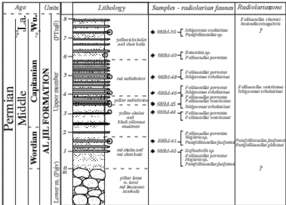
Figure 17- Stratigraphy of lower member and basal upper member of the Al Jil Formation at stops 3.1 and 3.2. (F. Cordey)
