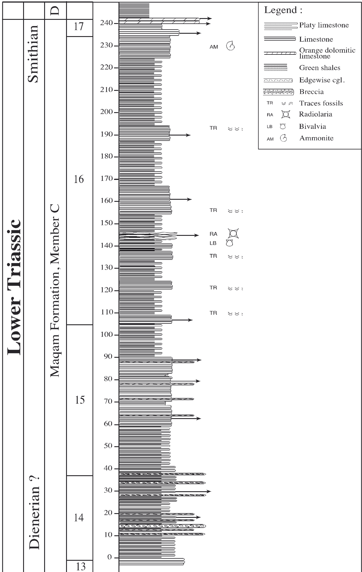
Figure 27- Measured section from the top of member C of the Maqam Formation (Wadi Shuyab).
