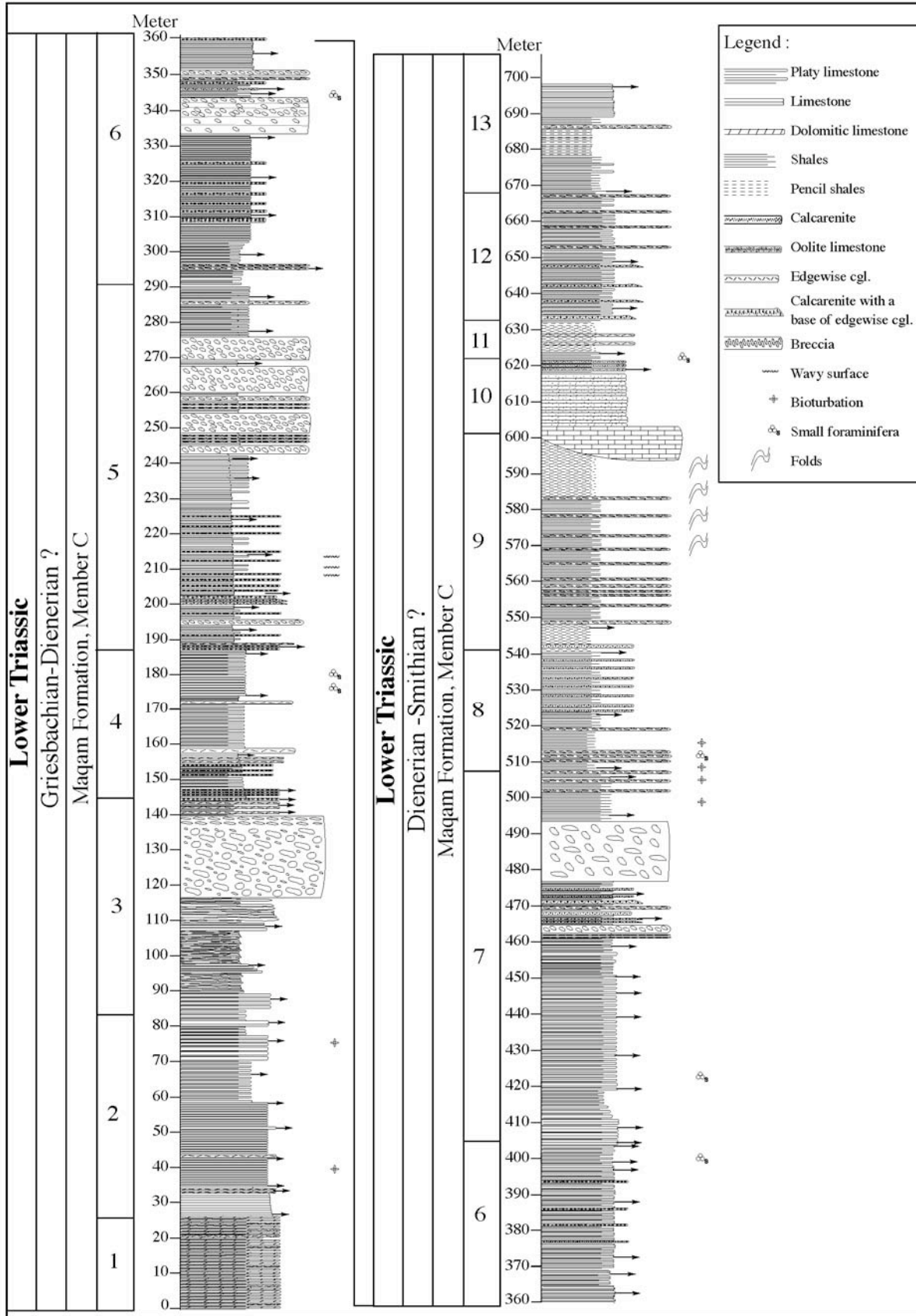
Figure 26- Measured section from the member C of the Maqam Formation (Wadi Maqam).
