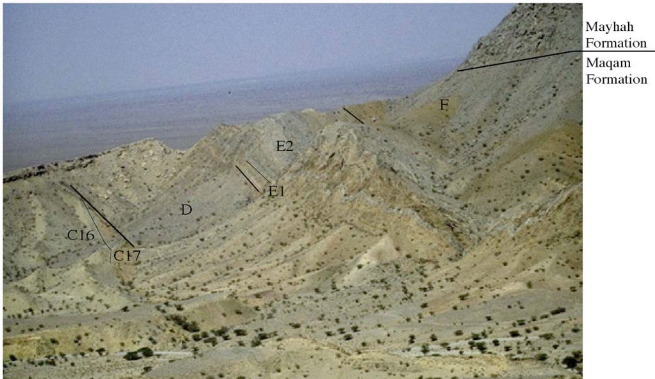
Figure 28- Upper part of the Maqam Formation (members D to F, Middle - Late Triassic).
