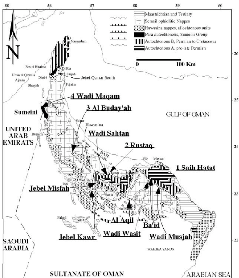
Fig. 3: Geological sketch of the Oman Mountains with the main visited localities (Excursions A01 and B01 = 1 - 4). Modified, from Pillevuit et al., (1997)
