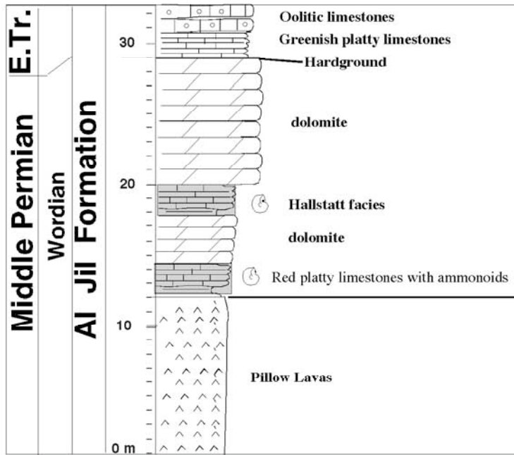
Figure 13- Stratigraphic sketch (section 1 of Rustaq) description in the text. (Modified after Pillevuit 1993, fig. 68).
