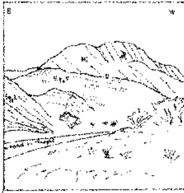
Figure 8 – Inverted, discordant sedimentary contact between the Hiyam Formation dolomite (Hi: upper part) and the Saiq Formation conglomerate (Sq 1 V: lower part), south bank of Wadi Aday)
