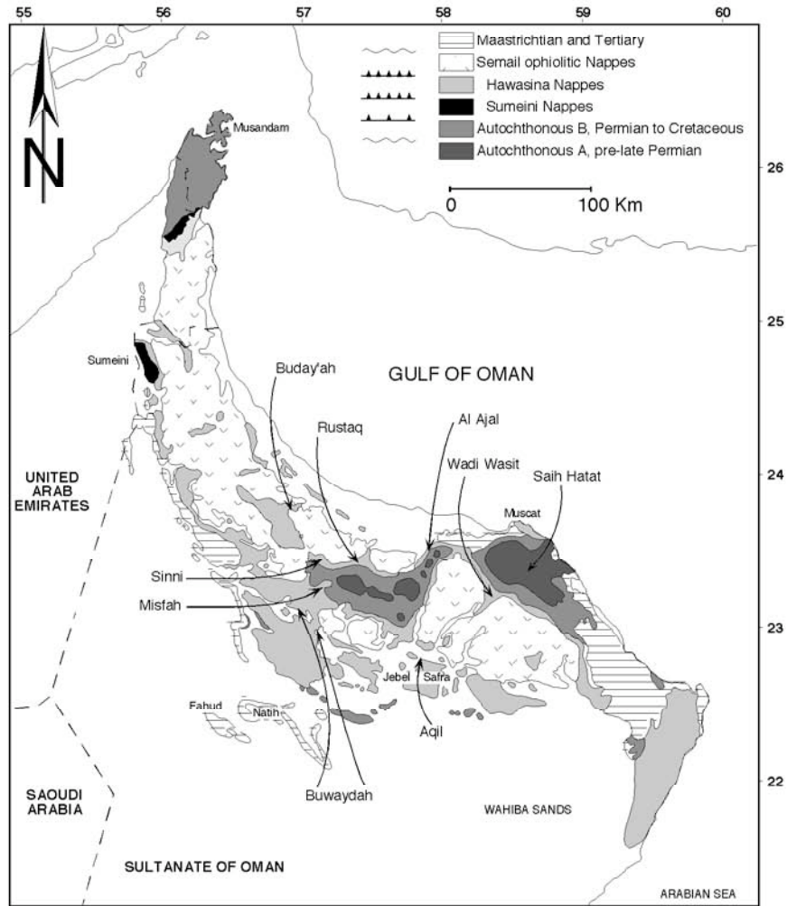
Fig. 5 -Geological sketch map of the Oman Mountains (after Glennie et al. 1974) with localities of Permian-Triassic volcanism cited in the text.
