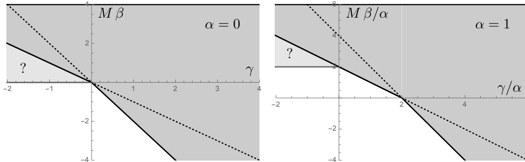
FIGURE 2. White (resp. dark grey) area corresponds to the domain in which \mathcal{E} is bounded (resp. unbounded) from below with \alpha = 0 on the left and \alpha = 1 on the right. Whether \mathcal{E} is bounded in the light grey domain or not is open so far.
