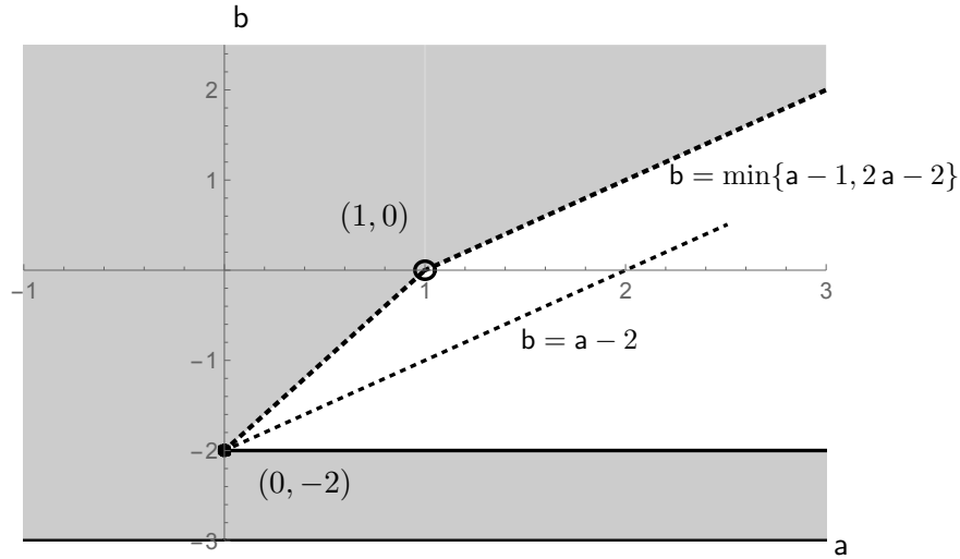
FIGURE 1. White (resp. grey) area corresponds to the domain in which (8) holds for some finite constant \mathcal{C}(a, b) (resp. \mathcal{C}(a, b) = -\infty ). We also know that \mathcal{C}(0, -2) = -(1 + \log \pi) and \mathcal{C}(1, 0) = -\infty , while the boundedness from below of \mathcal{F}_{a,b} is not known in the other threshold cases, i.e., for b = \min\{a - 1, 2a - 2\} with a \in (0, 1) \cup (1, +\infty) . On the dotted half-line b = a - 2 \geq -2 , optimality is achieved by \rho_\star and Inequality (8) corresponds to (5) with a = 2\tau , b = 2(\tau - 1) , and \tau \geq 0 .
