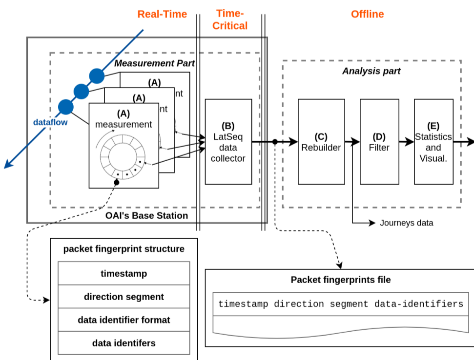
Fig.3 : LatSeq's architecture
