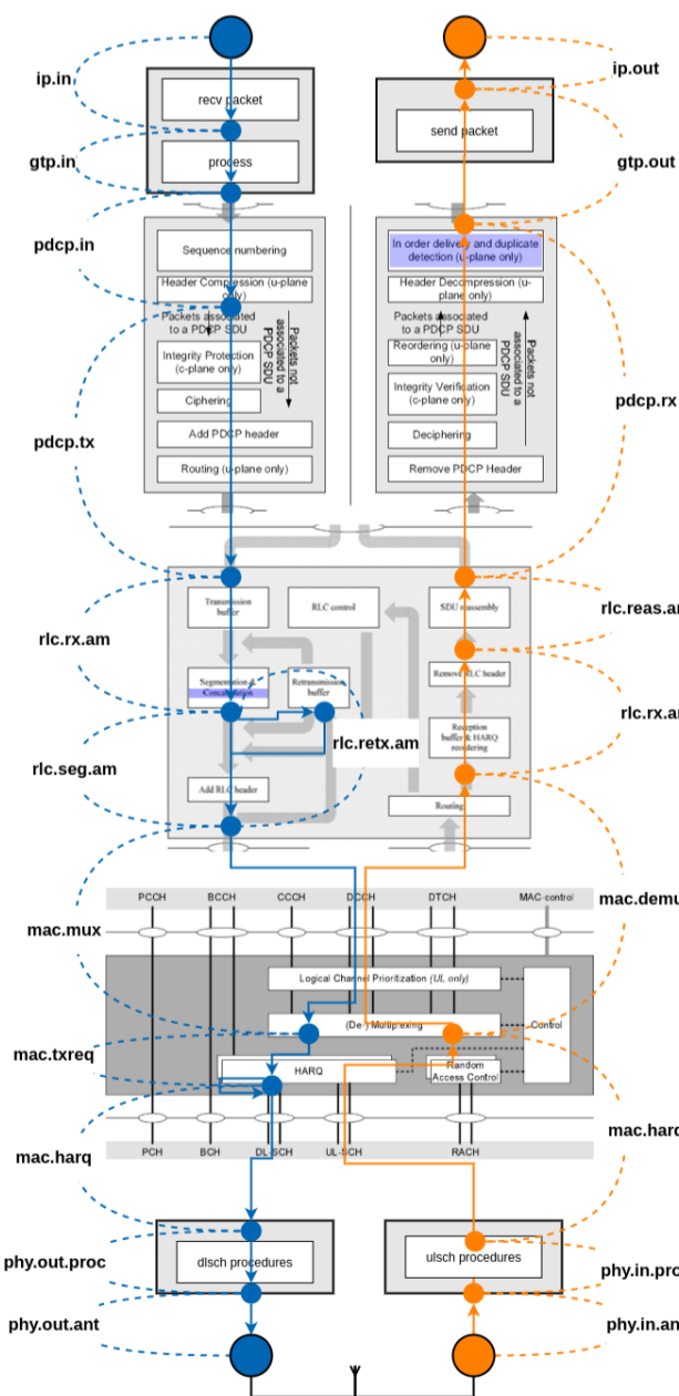
Fig.6 : LatSeq points on the OAI Base Station LTE stack
