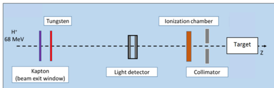
Figure 2. Proton beam setup. In this configuration, tungsten foil is used to homogenize the beam, for beam diameters greater than or equal to 1 cm. The target is a water tank or a mouse. Positions of each component are given in Table 1.
