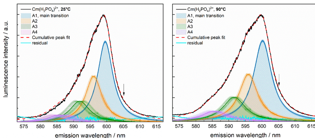
Figure 7. Extracted pure component emission spectra (black curves) of the \text{Cm}(\text{H}_2\text{PO}_4)_2^{2+} complex at 25 (left) and 90 °C (right) can be described with four Lorentzian peaks following the Boltzmann distribution depicting the emission transitions from the four crystal field states of the excited electronic level ( A_1 – A_4 ) back to the ground state. Errors expressed with 99.7% ( 3\sigma ) confidence of the fitted Lorentzian peak maxima and the fit residual (cyan traces) are included in the plots. Arrows indicate the part of the spectrum where the presence of an 8-fold coordinated \text{Cm}(\text{H}_2\text{PO}_4)_2^{2+} complex would be expected to appear.
