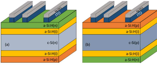
Figure 1: (a) n and (b) p-type stack TLM samples for extraction of the electron and hole contact parameters, respectively (texturing is not illustrated)
