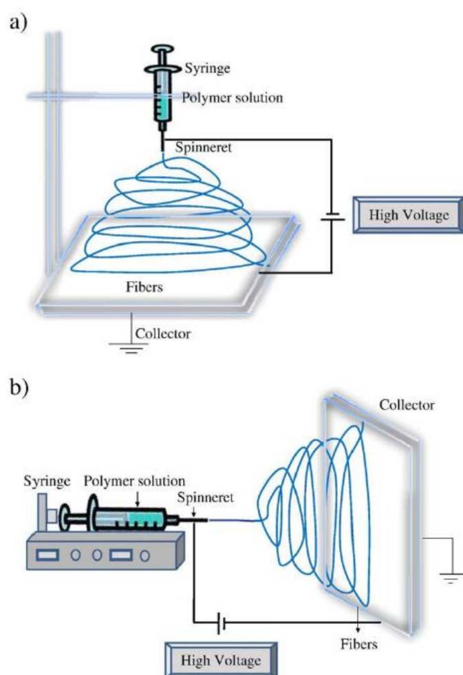
Figure 1. Schematic diagram of typical setups of an electrospinning apparatus: (a) vertical setup and (b) horizontal setup. Reprinted with permission from ref. [4]. Copyright 2010 Elsevier.
