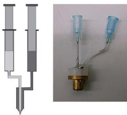
Figure 3. Left: A setup for coaxial electrospinning. Right: The experimental setup for coaxial electrospinning used in the laboratory of A. Greiner and J.H. Wendorff. Reprinted with permission from ref. [3]. Copyright 2007 from John Wiley and Sons.
