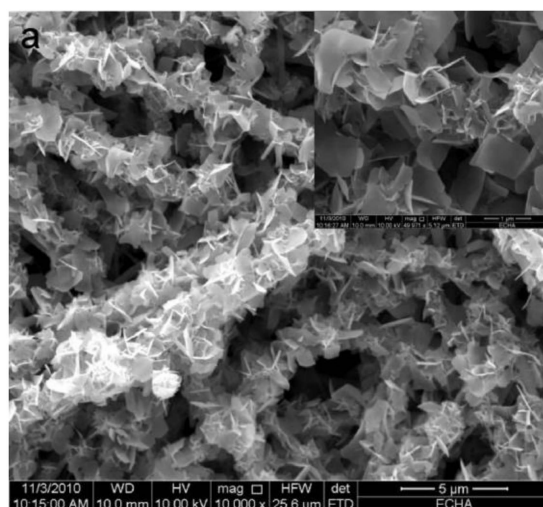
Figure 6. Surface of an electrospun cellulose scaffold mineralized in phosphate buffer saline for 1 week. Inset images reveal the higher magnification of the flake-like, high-surface-area, Ca-P minerals. Adapted with permission from ref. [89]. Copyright 2012 Elsevier.
