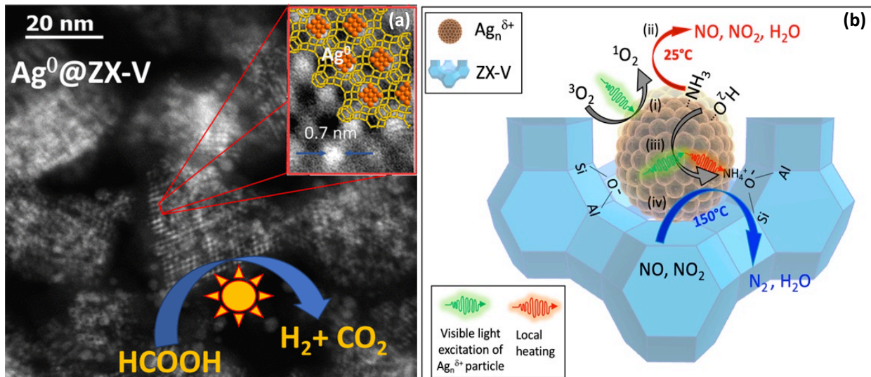
Fig. 8. a) The decomposition of formic acid into \text{H}_2 and \text{CO}_2 over \text{Ag}^0@ZX-V under visible light (liquid phase) and b) the proposed photo-SCR reaction mechanisms at RT and T=150^\circ\text{C} over \text{Ag}@ZX-V catalyst (El-Roz et al. , 2018; Hamoud et al. , 2019). Copyright 2018 and 2019 American Chemical Society and Elsevier, respectively. Reprinted with permission from El-Roz et al. 2018 and Hamoud et al. 2019.
