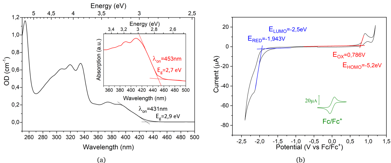
Fig. 3 (a) Absorption spectra of 10-OPIA in dichloromethane solution. Inset: Absorption spectrum in thin film form. (b) Cyclic voltammograms of 10-OPIA solution and Fc/Fc+ reference (vertical offset added for clarity).
