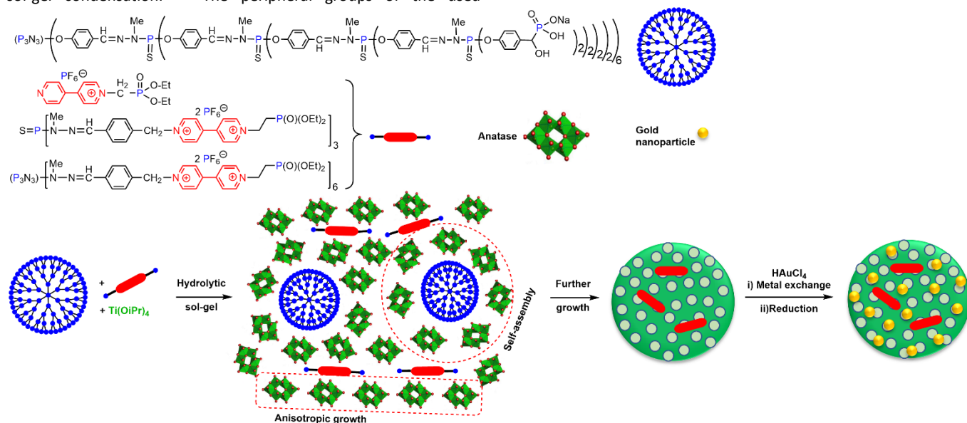
Scheme 5. Self-assembly and sol-gel polymerization of phosphonate-terminated dendrimers, soluble titanium-oxo species, and photoactive viologen units. Formation of porous anisotropic phosphonate-bridged-crystalline anatase materials hosts for dispersion and stabilization of small gold nanoparticles.
