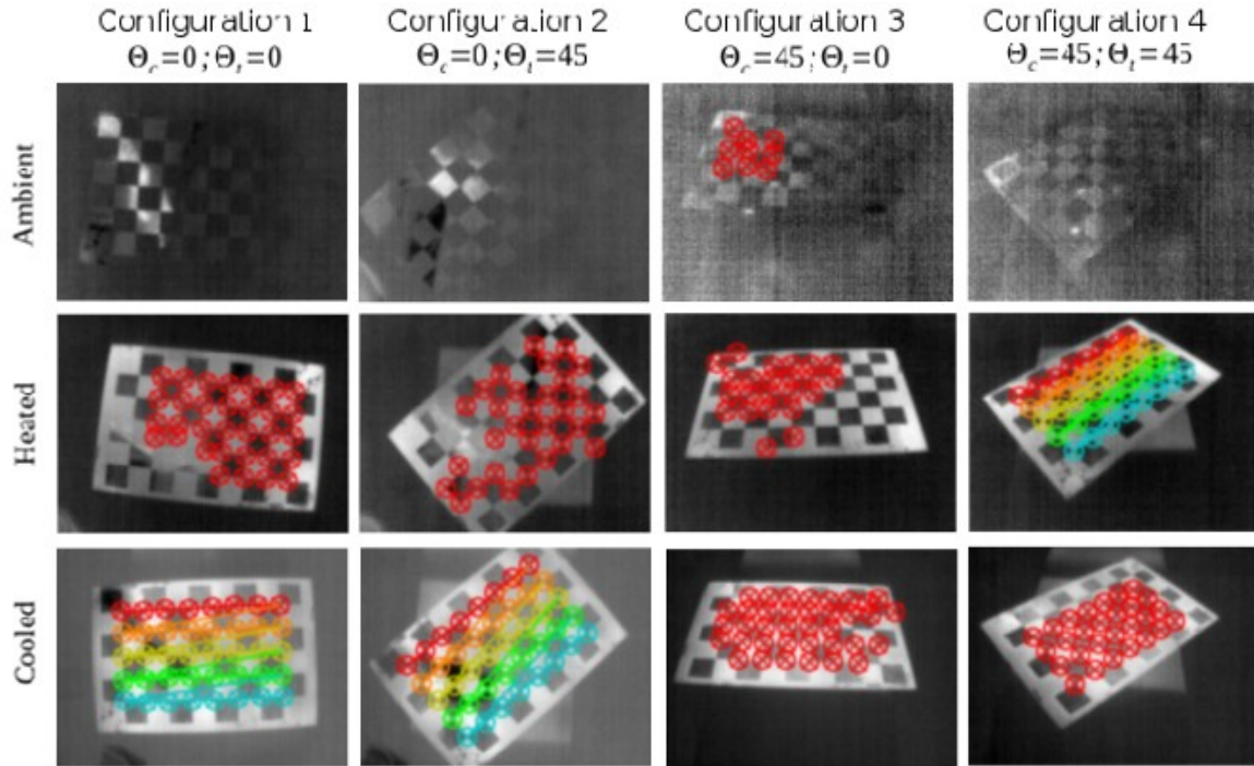
Fig. 5 : Detection points obtained by [8] on images acquired in each configurations.
