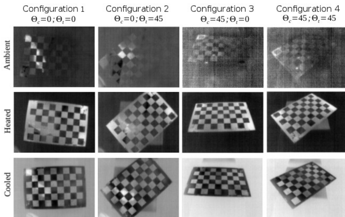
Fig. 4 : Examples of image acquired on each configuration and temperature situation : first line with an ambient target, second line with a heated target, third line with a cooled target.
