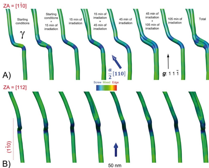
Figure 9: Detailed study of the glide evolution of dislocation segment \gamma with Burgers vector \frac{1}{2}[110] (green blue arrow) depicted in Fig. 7. A) evolution seen in the (110) glide plane. B) the (110) glide plane is edge-on. The colors correspond to the character from blue (screw) to red (edge). The diffraction vector is indicated by the black arrow.
