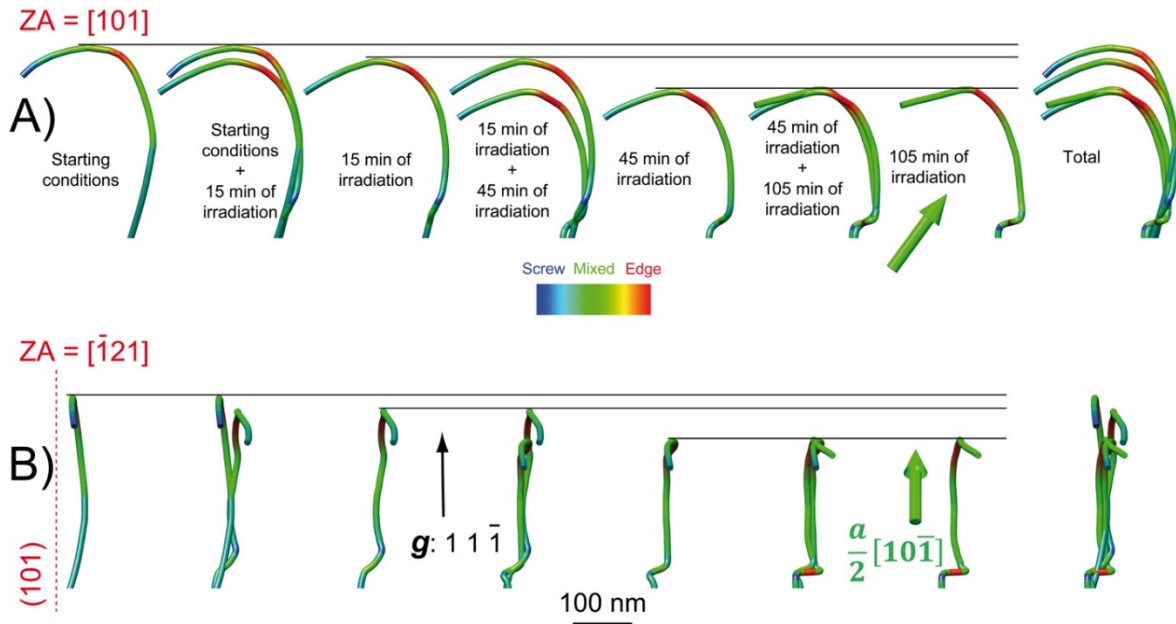
Figure 6. Detailed study of the glide evolution of the upper part of the dislocation described in Fig. 4 (in the red square of Fig. 2C)). A) evolution seen in the (101) glide plane. B) the (101) glide plane is edge-on. The colors correspond to the character from blue (screw) to red (edge). The diffraction vector is indicated by the black arrow. The Burgers vector \frac{1}{2}[10\bar{1}] is indicated by the thick green arrow.
