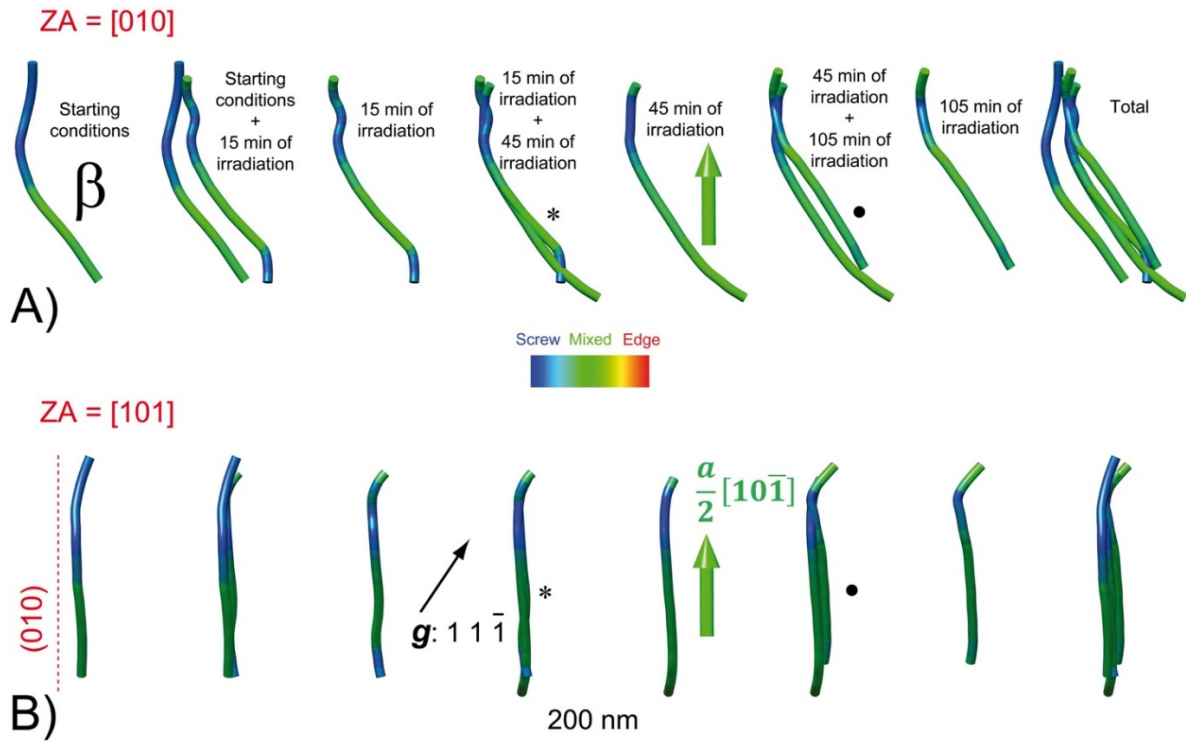
Figure 10. Detailed study of the glide evolution of dislocation segment \beta with Burgers vector \frac{1}{2}[10\bar{1}] (green thick arrow) depicted in Fig. 7. A) evolution seen in the (010) glide plane. B) the (010) glide plane is edge-on. The colors correspond to the character from blue (screw) to red (edge). The diffraction vector is indicated by the black arrow. The largest displacement is observed during the first stage of the experiment, then the dislocation stagnates during the additional 45 min of irradiation (*). Finally, during the last 105 min of irradiation, the dislocation moves slightly outside the glide plane by climb ( \bullet ).
