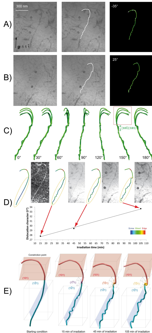
Figure 4. Evolution of a \frac{1}{2}[10\bar{1}] dislocation under electron irradiation. The dislocation is seen at -35^\circ in A) and 25^\circ in B) (both at 45 min irradiation). Left is the raw image, in the middle is the tracing superimposed to it and right is the tomographic model. C) Superimposition of the four tomographic models at 0, 15, 45 and 105 min irradiation time at 650^\circ\text{C} . Evolution of the upper part in the red square is presented in greater details in Fig. 6. D) shows the dislocation character with a color gradient (inset) for the dislocation viewed at 0^\circ . The graph shows that the average dislocation character evolves linearly with irradiation time toward more edge components. E) Indexing of the planes containing the dislocations segments. The upper part (in red) is contained in (101) while the lower part (in blue) is in (\bar{1}\bar{2}1) revealing cross-slip of the initial configuration. The evolution of the segment located in between is shown. The 3D evolution of the blue segment is described in more details in Fig. 11A.
