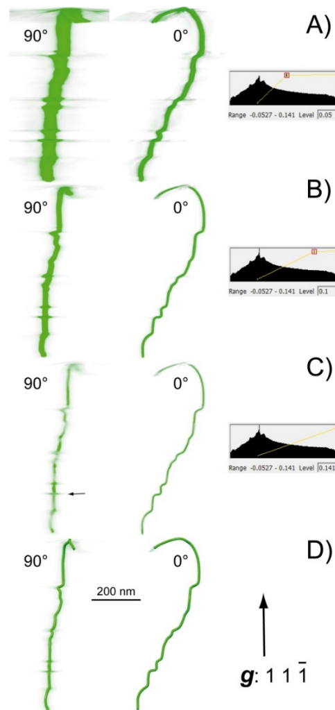
Figure 1. Methodology used to trace dislocation lines with the Chimera software considering the uncertainty related to the missing wedge. A) raw reconstructed volume (from Figure 4) for two projected angles ( 90^\circ and 0^\circ ) with a gray value of 0.05 (32-bit image) the ribbon resulting from the missing wedge is clearly visible at 90^\circ . B) with a gray value of 0.1, the extension of the ribbon is reduced. C) with the highest accessible gray value (0.141), the position of the dislocation can be determined with accuracy, even at 90^\circ . D) superimposing the traced dislocation on the raw reconstructed volume from Figure 4C (45 min irradiation). The diffraction vector is indicated by the vertical black arrow.
