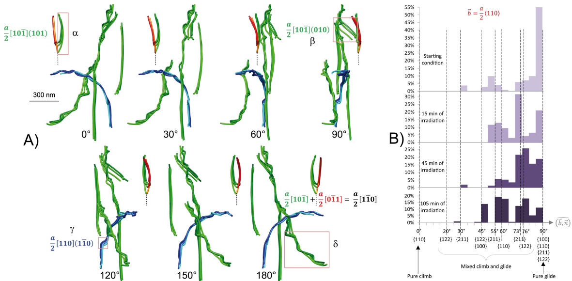
Figure 7. A) Evolution with irradiation of a zone containing seven dislocations (in contrast). Seven orientations are represented and the four tomographic models are superimposed. A \frac{1}{2}[1\bar{1}0] dislocation resulting from a junction which is out of contrast is represented by a dashed line. Movie S2 shows how this microstructure evolves continuously with irradiation. Evolution of dislocations \alpha , \beta and \gamma are presented in more details in Figs. 8, 10 and 9 respectively. B) Bar graph presenting the cumulated frequencies of planes containing dislocation segments as a function of the angle between the plane normal and the Burgers vectors. The gliding configurations are on the right (90°), the pure climb is on the left (0°). The intermediate configurations correspond to mixed climb.
