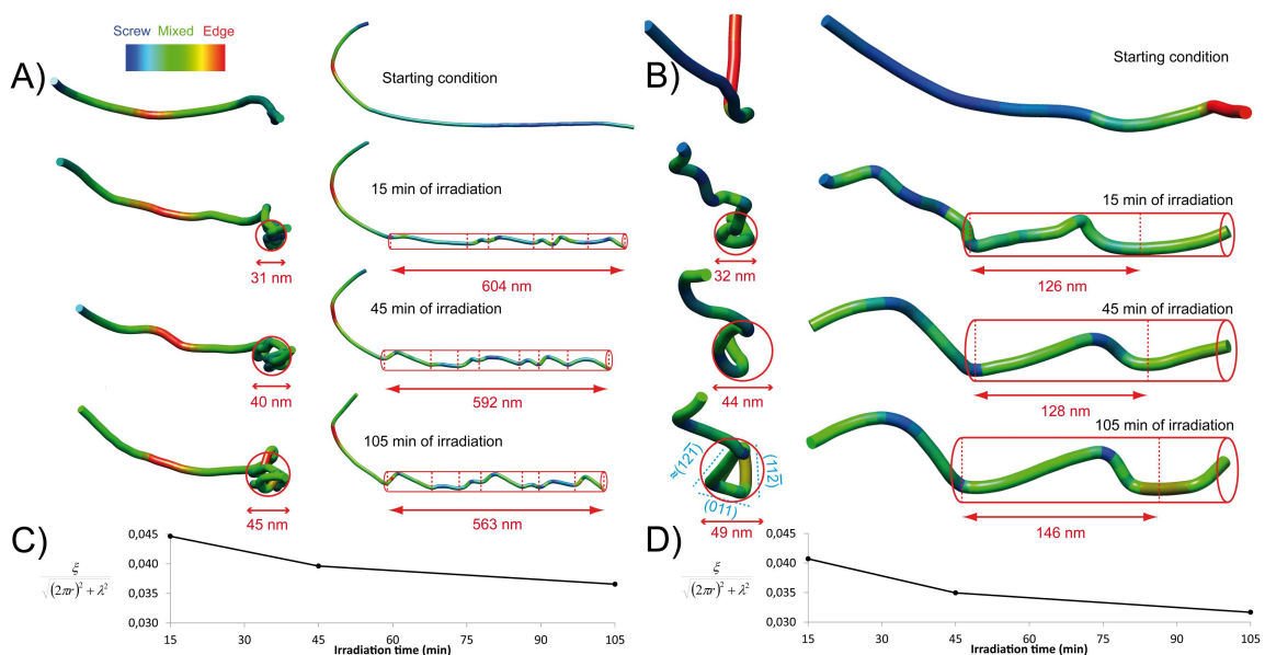
Figure 11. Helix formation. A) dislocation of Fig. 4 seen along the direction of the long initially relatively straight segment (left) and perpendicularly (right) B) same for the segment marked by \delta in Fig. 7. C) and D) represent (for A) and B) respectively) the evolution during irradiation of the geometrical parameter representative of the oversaturation of point defects (see text).
