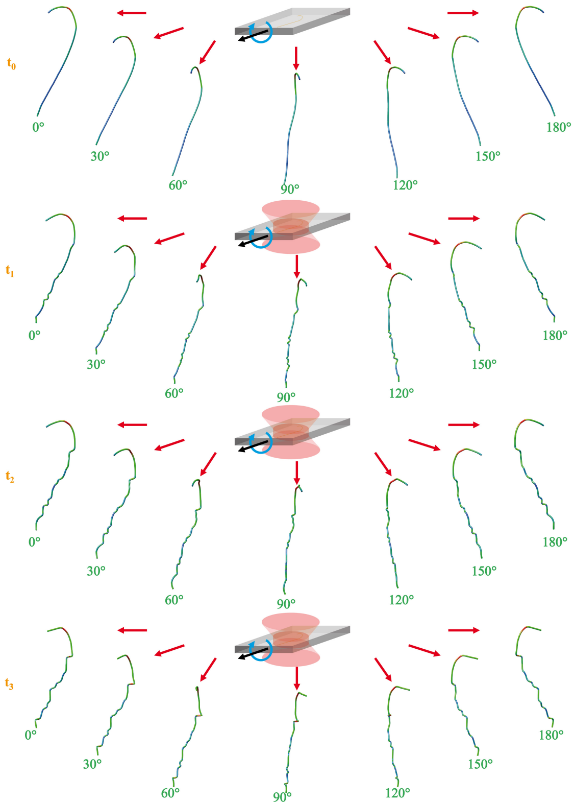
Figure 3. Schematic representation of time-resolved 4D electron tomography of a dislocation undergoing annealing and electron irradiation. A) t_0 represents initial conditions where the 3D structure of a given dislocation is presented under seven viewing angles ranging from 0 to 180°. B) t_1 corresponds to 15 min of irradiation at 650°C corresponding to an electron dose of 3.0 \times 10^7 electron.nm -2 . C) t_2 corresponds to 45 min of irradiation at 650°C (electron dose 9.0 \times 10^7 electron.nm -2 ). D) t_3 corresponds to 105 min of irradiation at 650°C (electron dose 21.1 \times 10^7 electron.nm -2 ). Movie S1 displays a continuous evolution with time of this dislocation viewed in 3D.
