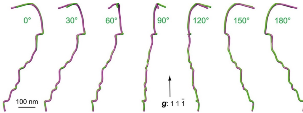
Figure 2. Comparison between the reconstructed green volume obtained with 10 projected images ( -35^\circ , -25^\circ , -20^\circ , -15^\circ , -5^\circ , 0^\circ , 5^\circ , 10^\circ , 15^\circ and 25^\circ ) and the reconstructed purple volume obtained with 2 projected images ( -35^\circ and 25^\circ ). The diffraction vector is indicated by the black arrow.
