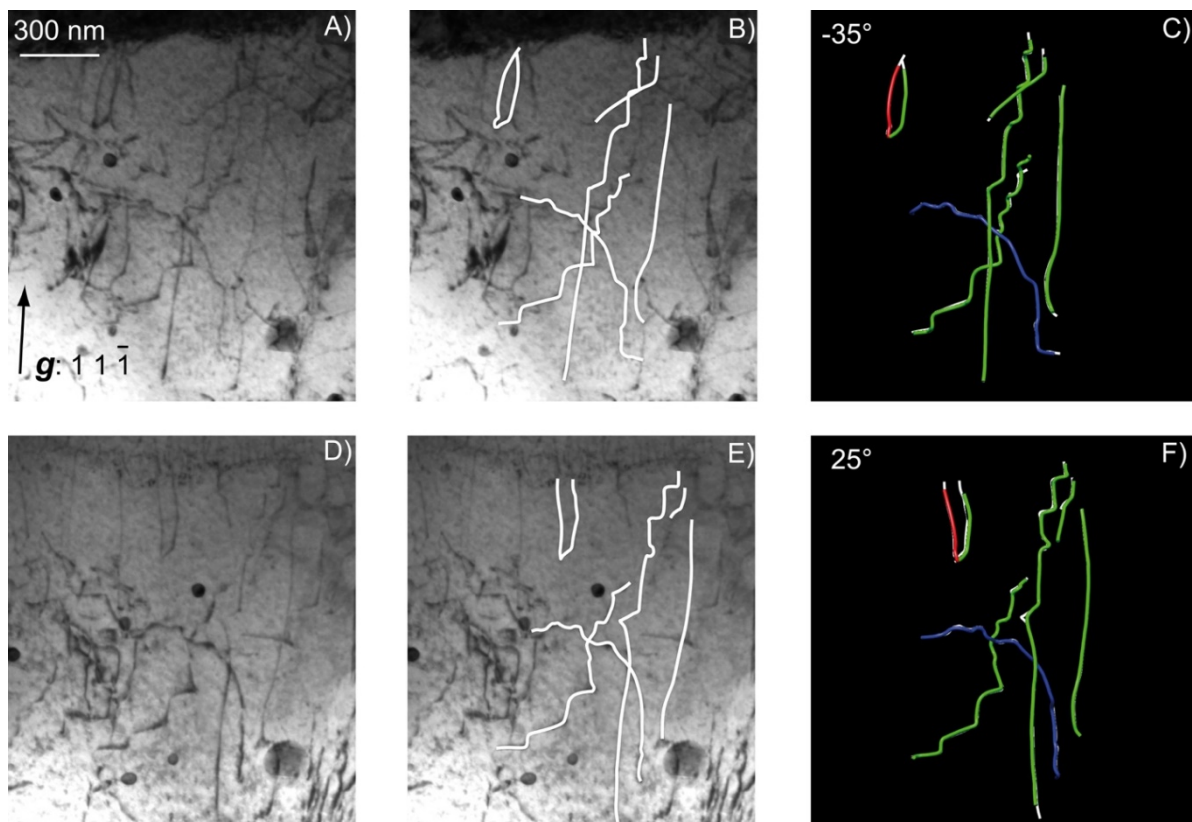
Figure 5. Illustration of the main steps of tomographic reconstruction for the seven dislocations presented in Fig. 7 (Irradiation time 105 min). Left is the raw image, in the middle is the tracing superimposed to it and right is the tomographic model superimposed to the tracing. A), B) and C) correspond to -35^\circ . D), E) and F) correspond to 25^\circ .
