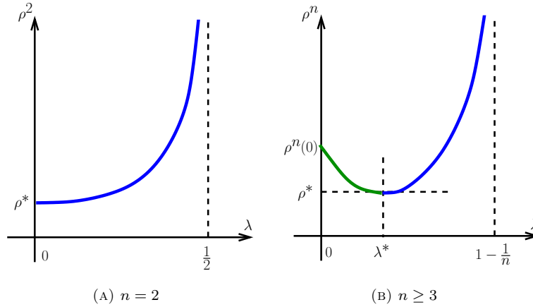
FIGURE 1. Graphical representation of the function \lambda \mapsto \rho^n(\lambda) (after [57]). (a) case n = 2 . (b) case n \geq 3 . The portions of the curves that correspond to stable equilibria are in blue, the unstable ones, in green.
