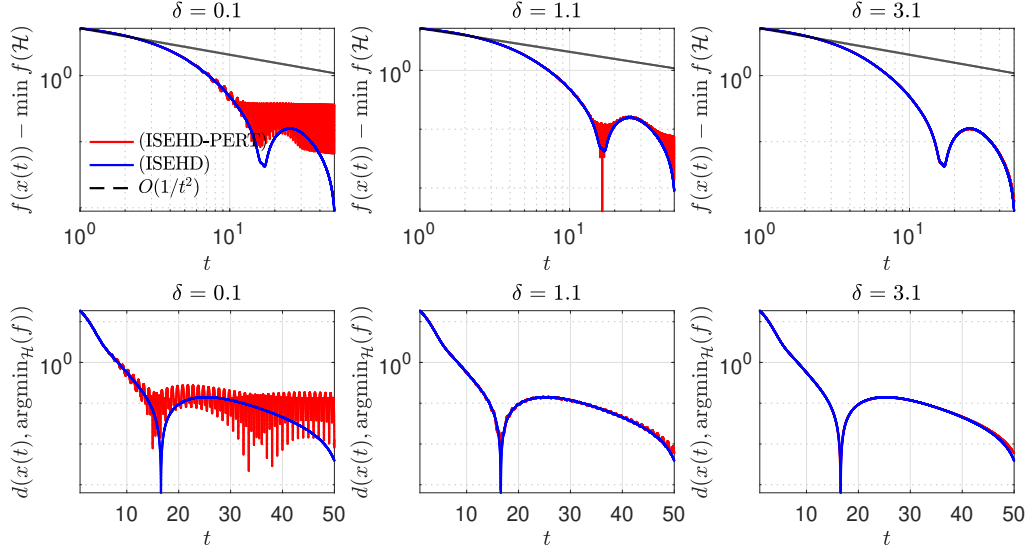
(a) Explicit Hessian damping: smooth function
