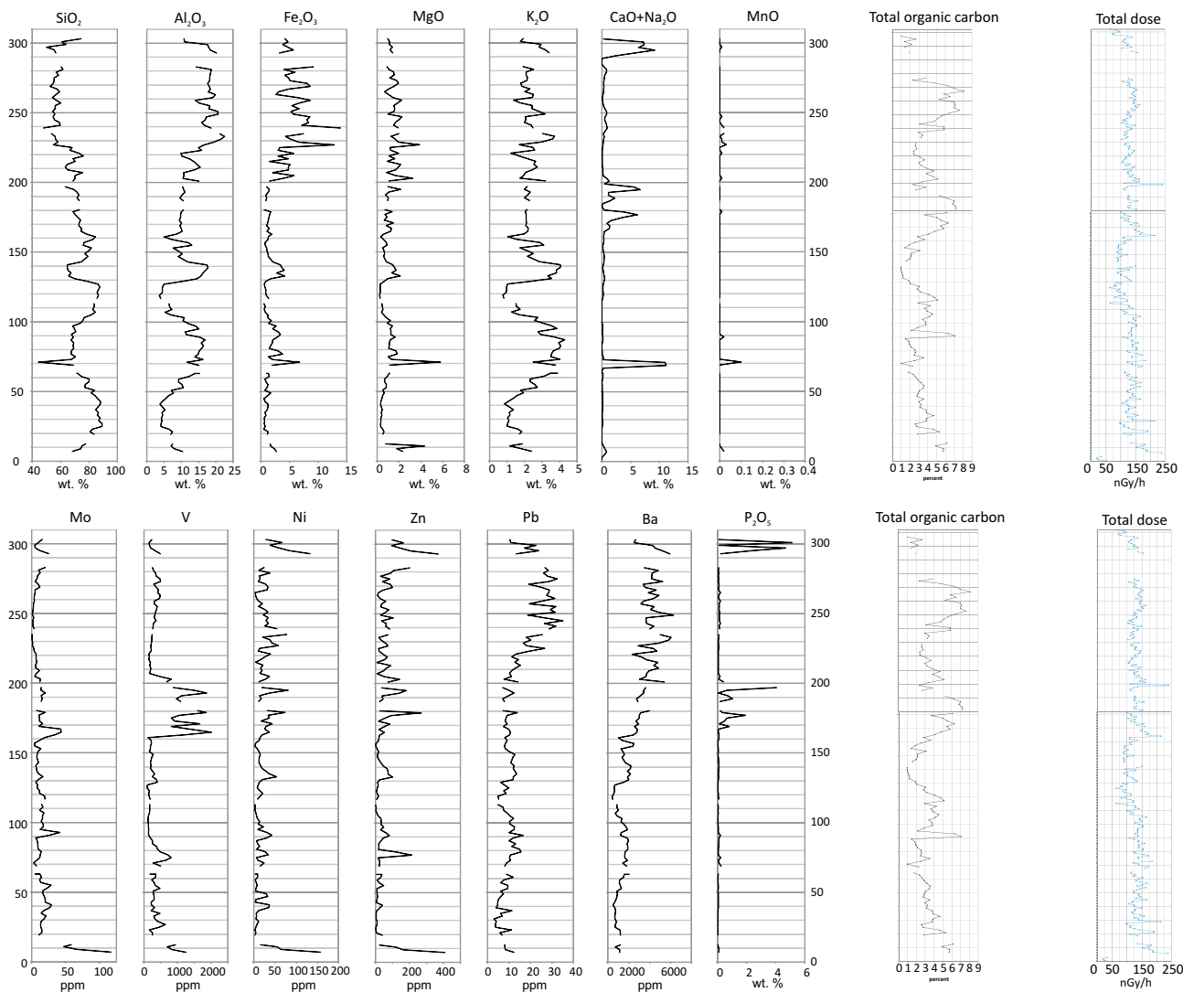
Figure 16. Major, minor and trace element abundances across the section of Besa River Formation measured in the Stone Mountain area by Ferri et al. (2012).
