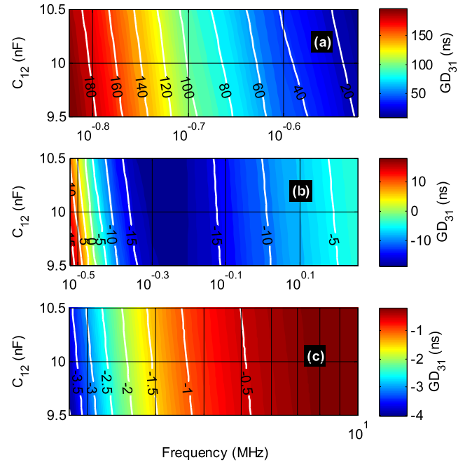
FIGURE 14. Mappings of GD_{31} zoomed in (a) [150 \text{ kHz}, 300 \text{ kHz}] , (b) [300 \text{ kHz}, 1.8 \text{ MHz}] and (c) [1.8 \text{ MHz}, 10 \text{ MHz}] versus (f, C_{12}) .
