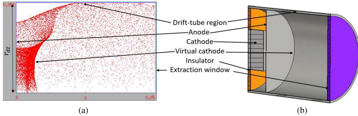
Figure 19. Vircator model simulated using (a) XOOPIC and (b) CST-PS.
