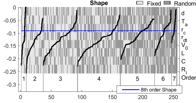
Figure 10. Computed shape parameter for each set of the 256 possible combinations as a result of the RVs (vertical scale stands for the RVs combination). Shape parameter values have been sorted from lower to higher values within each combination orders 1–7.
