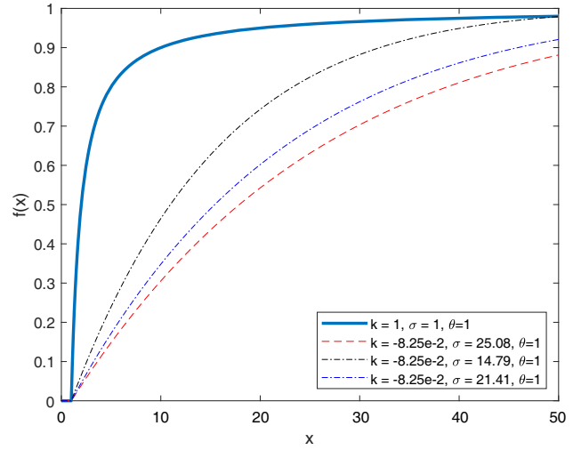
Figure 6. Three cumulative distribution functions for different scale parameters of the GPD and a fixed shape value.
