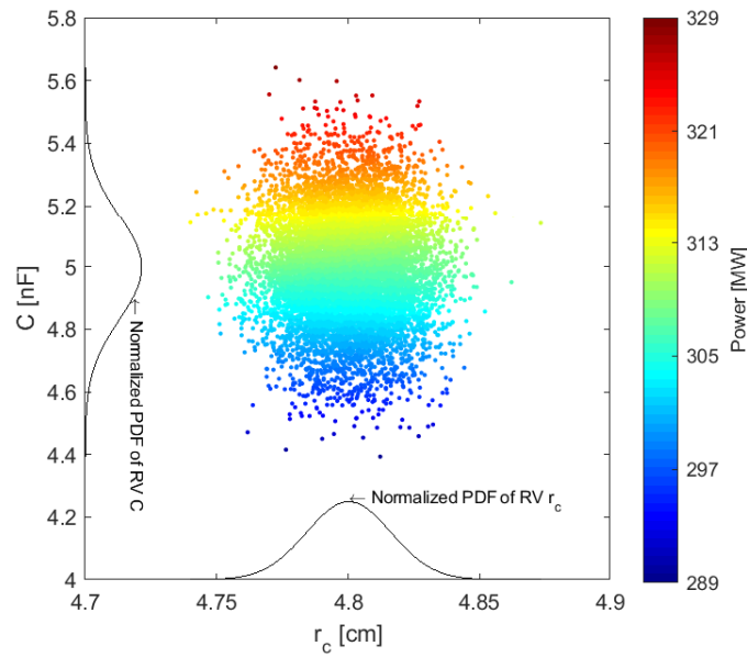
Figure 3. Monte-Carlo simulation — Computed peak power with r_c and C_s as RVs while d , T_a , r_{dt} , V_0 , L_s , and R_s are fixed at their mean value.
