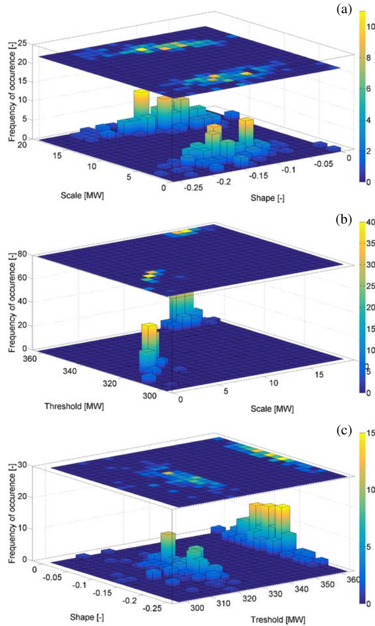
Figure 9. Bivariate histograms of the pairs of parameters. (a) Shape and scale. (b) Scale and threshold. (c) Threshold and shape.
