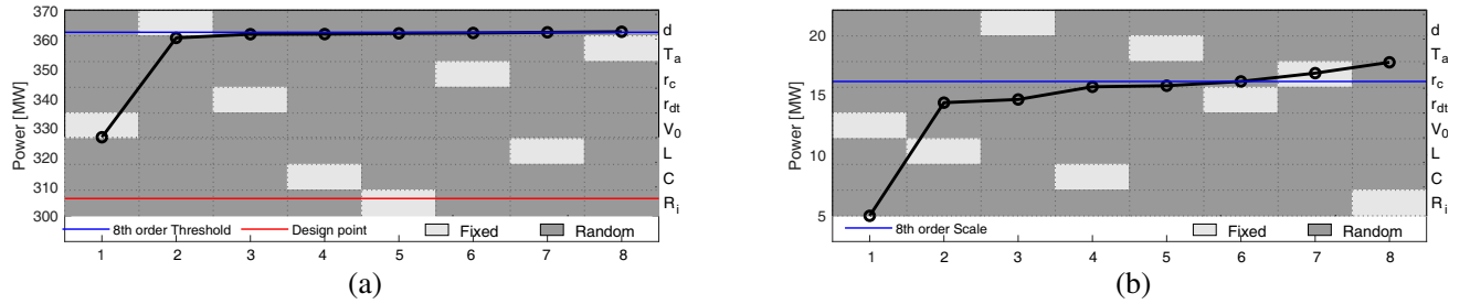
Figure 18. (a) Sorted threshold and (b) scale values obtained for 7 RVs.
