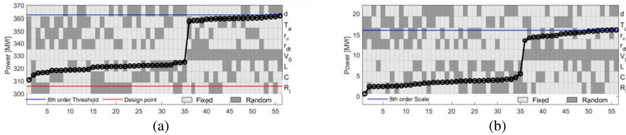
Figure 14. (a) Sorted threshold and (b) scale values obtained for 3 RVs.
