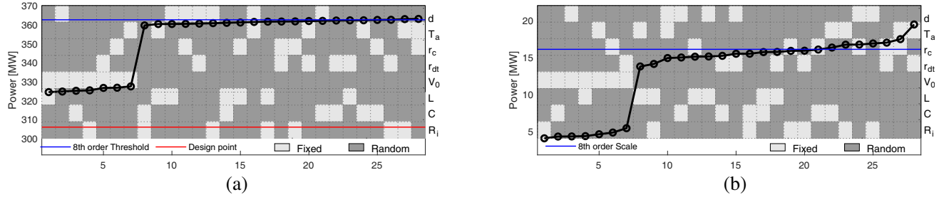
Figure 17. (a) Sorted threshold and (b) scale values obtained for 6 RVs.
