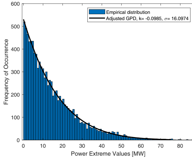
Figure 7. Histogram of the peak power extreme values considering the 8 RVs and the inferred GPD.
