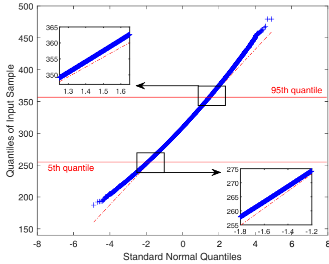
Figure 4. Quantile to quantile plot of the estimated power values against the theoretical quantile values of a standard normal distribution.
