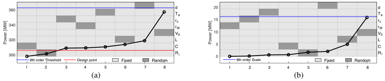
Figure 12. (a) Sorted threshold and (b) scale values obtained for 1 RV.
