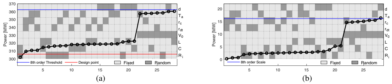
Figure 13. (a) Sorted threshold and (b) scale values obtained for 2 RVs.
