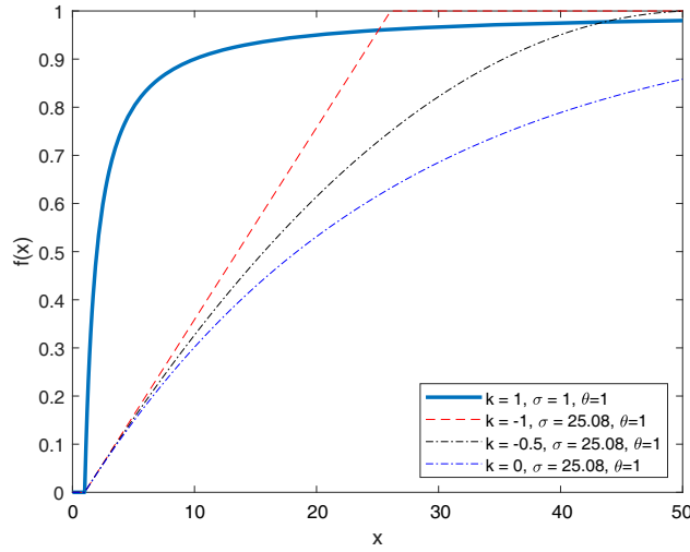
Figure 5. Three cumulative distribution functions for different shape parameters of the GPD with a fixed scale value.
