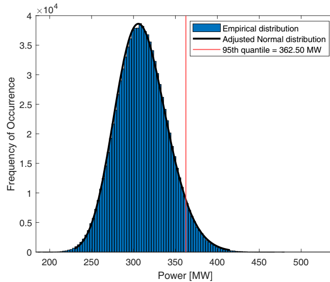
Figure 2. Histogram of 1,000,000 Monte-Carlo computations of the output peak power considering the 8 RVs.
