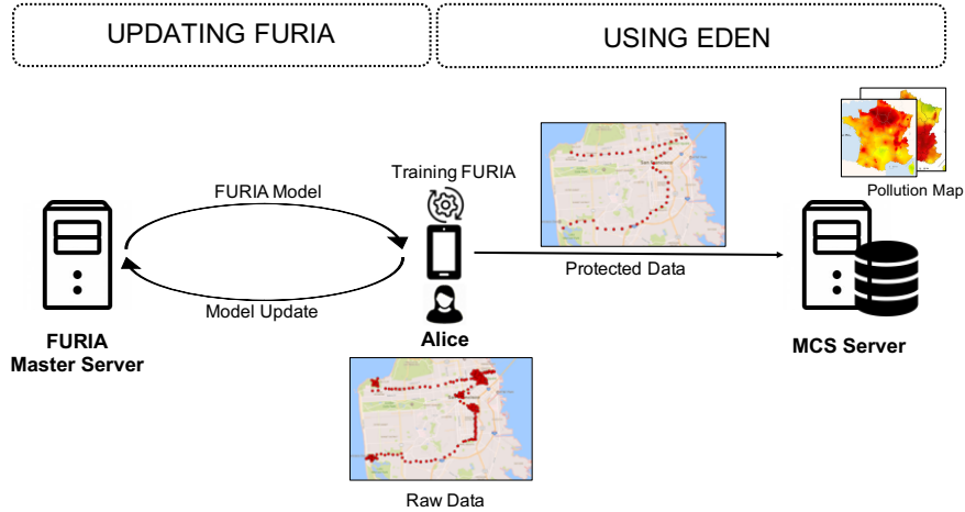
Fig. 2: System Architecture
