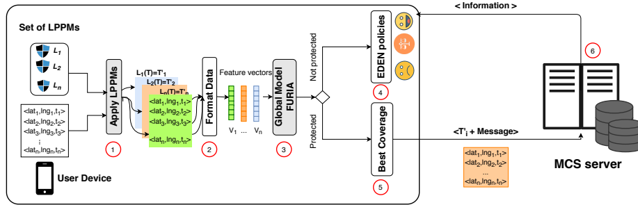
Fig. 5: EDEN architecture
