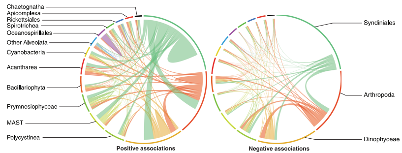
Figure 3.1: Community structure found in photic zone interactome. Top 15 interacting taxon groups are depicted as colored segments in which ribbons connecting two segments indicate co-presence and exclusion. Links are dominated by the obligate parasites syndiniales and by Arthropoda and Dinophyceae. Source: Lima-Mendez et al. 2015.
