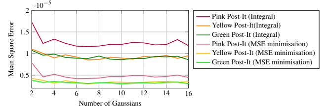
Figure 5: Mean squared error between the measured datasets and the reconstruction with different number of Gaussians and different weighting factors. We use the same mixture for both techniques to compute the scaling factor. From 3 Gaussians, we observe a significant drop in the reconstruction error using the MSE metric. Adding additional Gaussians does not significantly reduce MSE.
