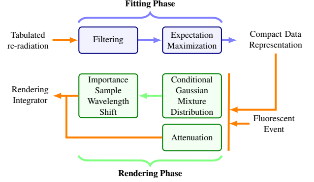
Figure 3: Representation of our pipeline. We model the input re-radiation with a GMM in the fitting phase and then use it in the renderer. In the rendering phase, we importance sample the new wavelength according to the GMM.
