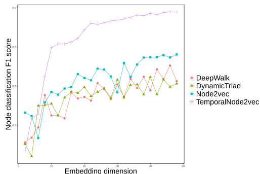
Fig. 1: Node classification on AMiner 3 dataset
