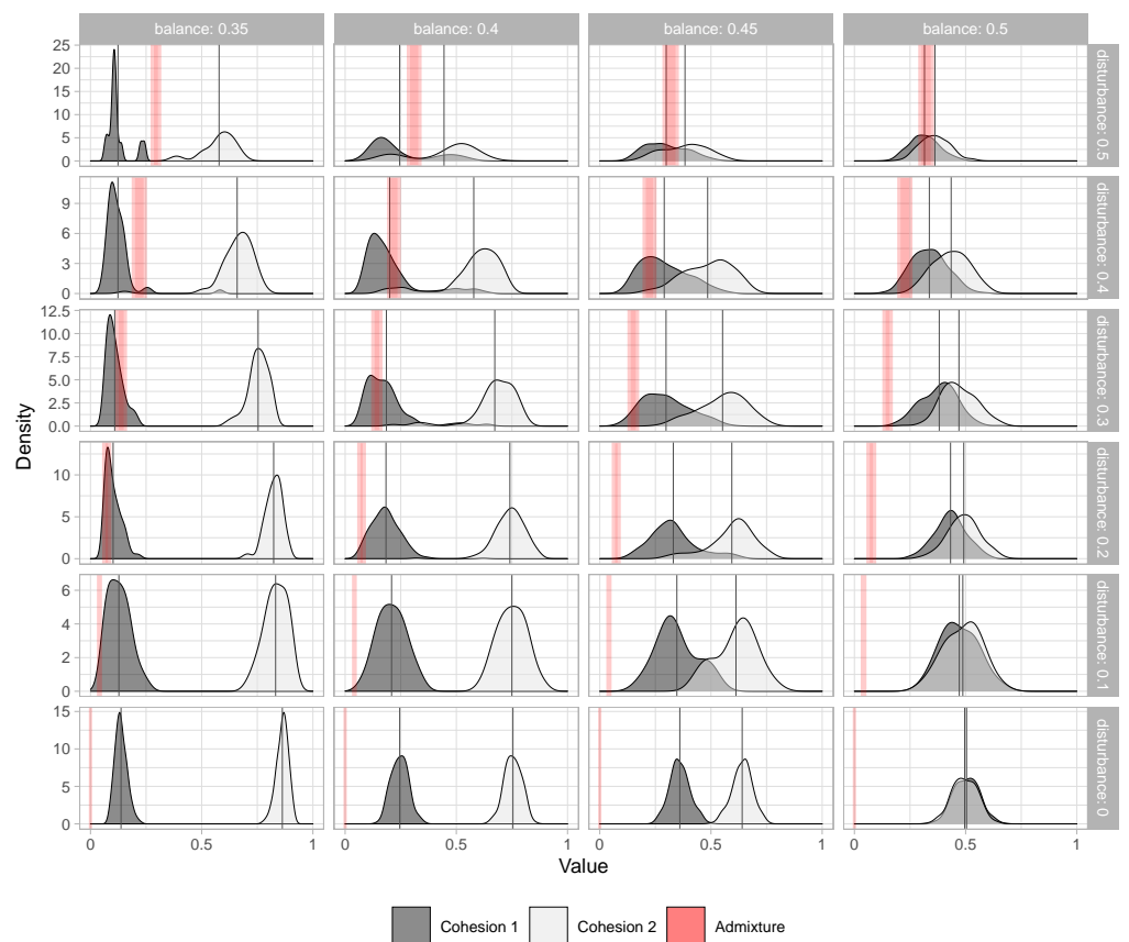
Figure 10. Density of the cohesion values for layers 1 and 2 of the simulated graphs (30 objects, 100 fragments) for different balance (columns) and disturbance (rows) parameters (6000 graphs). The black vertical lines give the mean cohesion values. Admixture is summarised by the red shades (representing the interquartile range of the values) and is also indicated by the positions of the cohesion values: the smaller the values, the more the layers are mixed. The reading is similar to the reading of Table 1. E.g., the upper left case corresponds to two layers with unequal cohesion values and high admixture.
